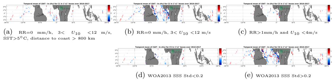
Figure 12: Temporal mean gridded over spatial boxes of size 1^\circ \times 1^\circ of \Delta SSS (SMOS-L3-CATDS-CECOS-IFREMER-V2-1DAY-0.5DEG - TSG-GOSUD-Research-vessel) for 5 different subdatasets corresponding to: RR=0 mm/h, 3 < U_{10} < 12 m/s, SST > 5°C, distance to coast > 800 km (a), RR=0 mm/h, 3 < U_{10} < 12 m/s (b), RR > 1mm/h and U_{10} < 4 m/s (c), WOA2013 SSS Std < 0.2 (d), WOA2013 SSS Std > 0.2 (e).
