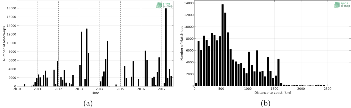
Figure 1: Number of match-ups between TSG-GOSUD-Research-vessel and SMOS-L3-CATDS-CECOS-IFREMER-V2-1DAY-0.5DEG SSS as a function of time (a) and as function of the distance to coast (b) over the Equatorial Ocean 10N-10S Pi-MEP region and for the full satellite product period.
