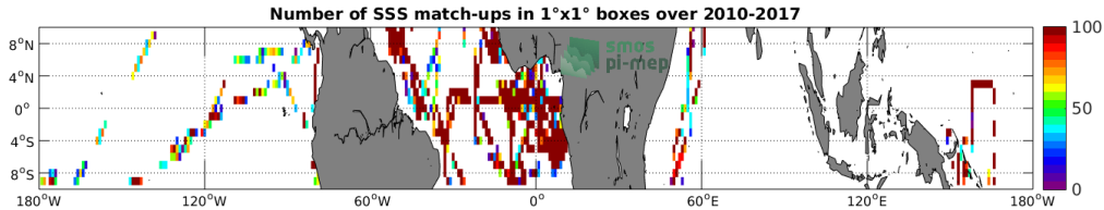
Figure 4: Number of SSS match-ups between TSG-GOSUD-Research-vessel SSS and the SMOS-L3-CATDS-CECOS-IFREMER-V2-1DAY-0.5DEG SSS product for the Equatorial Ocean 10N-10S Pi-MEP region over 1°x1° boxes and for the full satellite product period.
