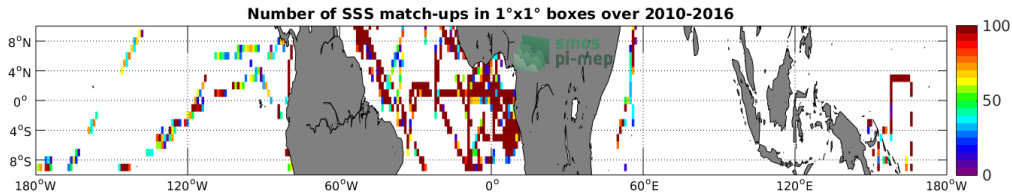
Figure 4: Number of SSS match-ups between TSG-GOSUD-Research-vessel SSS and the SMOS-L3-CATDS-CECOS-IFREMER-V2-1DAY-0.5DEG SSS product for the Equatorial Ocean 10N-10S Pi-MEP region over 1^\circ \times 1^\circ boxes and for the full satellite product period.
