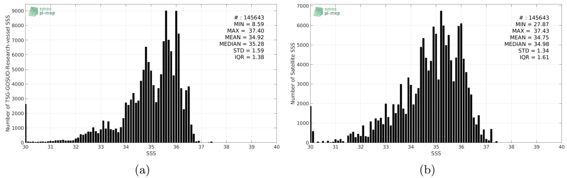
Figure 2: Histograms of SSS from TSG-GOSUD-Research-vessel (a) and SMOS-L3-CATDS-CECOS-IFREMER-V2-1DAY-0.5DEG (b) considering all match-up pairs per bins of 0.1 over the Equatorial Ocean 10N-10S Pi-MEP region and for the full satellite product period.
