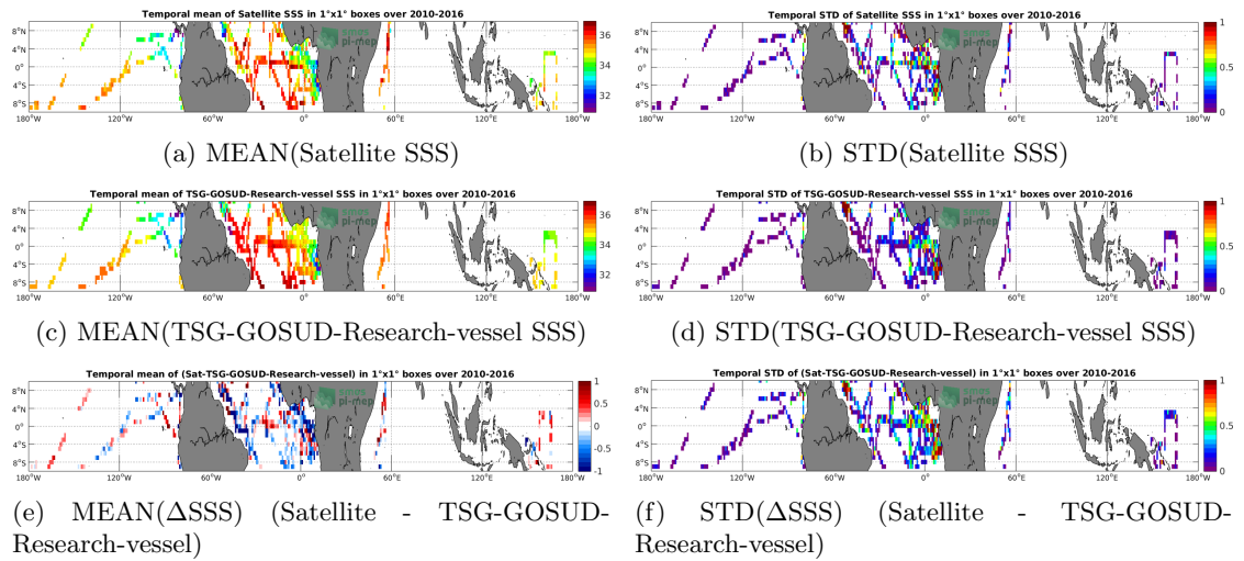
Figure 6: Temporal mean (left) and STD (right) of SSS from SMOS-L3-CATDS-CECOS-IFREMER-V2-1DAY-0.5DEG (top), TSG-GOSUD-Research-vessel (middle), and of \Delta SSS (Satellite - TSG-GOSUD-Research-vessel). Only match-up pairs are used to generate these maps.
