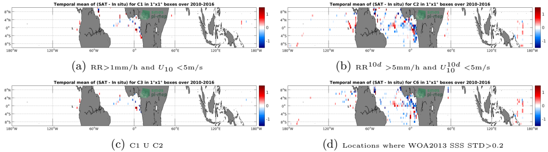
Figure 12: Temporal mean gridded over spatial boxes of size 1^\circ \times 1^\circ of \Delta SSS (SMOS-L3-CATDS-CECOS-IFREMER-V2-1DAY-0.5DEG - TSG-GOSUD-Research-vessel) for 4 different subdatasets corresponding to:RR>1mm/h and U_{10} < 5\text{m/s} (a), RR^{10d} > 5\text{mm/h} and U_{10}^{10d} < 5\text{m/s} (b), C1 U C2 (c),Locations where WOA2013 SSS STD>0.2 (d).
