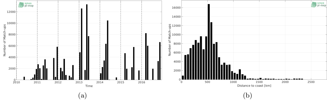
Figure 1: Number of match-ups between TSG-GOSUD-Research-vessel and SMOS-L3-CATDS-CECOS-IFREMER-V2-1DAY-0.5DEG SSS as a function of time (a) and as function of the distance to coast (b) over the Equatorial Ocean 10N-10S Pi-MEP region and for the full satellite product period.
