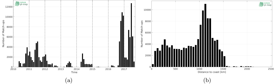
Figure 1: Number of match-ups between Surface drifters and SMOS-L3-CATDS-CECOS-IFREMER-V2-1DAY-0.5DEG SSS as a function of time (a) and as function of distance to coast (b) over the Equatorial Ocean 10N-10S Pi-MEP region and for the full satellite product period.
