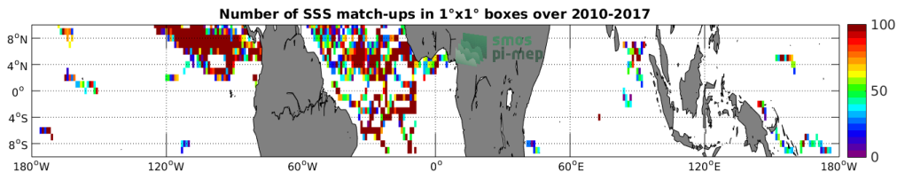
Figure 3: Number of SSS match-ups between Surface drifters SSS and the SMOS-L3-CATDS-CECOS-IFREMER-V2-1DAY-0.5DEG SSS product for the Equatorial Ocean 10N-10S Pi-MEP region over 1°x1° boxes and for the full satellite product period.
