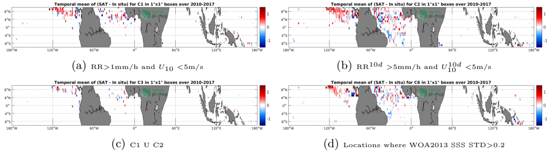
Figure 11: Temporal mean gridded over spatial boxes of size 1^\circ \times 1^\circ of \Delta SSS (SMOS-L3-CATDS-CECOS-IFREMER-V2-1DAY-0.5DEG - Surface drifters) for 4 different subdatasets corresponding to: RR>1mm/h and U_{10} < 5\text{m/s} (a), RR^{10d} > 5\text{mm/h} and U_{10}^{10d} < 5\text{m/s} (b), C1 U C2 (c), Locations where WOA2013 SSS STD>0.2 (d).
