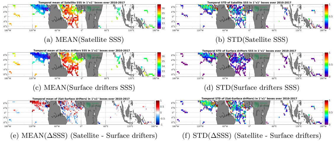
Figure 5: Temporal mean (left) and STD (right) of SSS from SMOS-L3-CATDS-CECOS-IFREMER-V2-1DAY-0.5DEG (top), Surface drifters (middle), and of \Delta SSS (Satellite - Surface drifters). Only match-up pairs are used to generate these maps.
