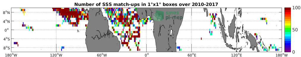
Figure 3: Number of SSS match-ups between Surface drifters SSS and the SMOS-L3-CATDS-CECOS-IFREMER-V2-1DAY-0.5DEG SSS product for the Equatorial Ocean 10N-10S Pi-MEP region over 1^\circ \times 1^\circ boxes and for the full satellite product period.
