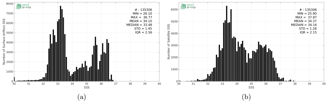
Figure 2: Histograms of SSS from Surface drifters (a) and SMOS-L3-CATDS-CECOS-IFREMER-V2-1DAY-0.5DEG (b) considering all match-up pairs per bins of 0.1 over the Equatorial Ocean 10N-10S Pi-MEP region and for the full satellite product period.
