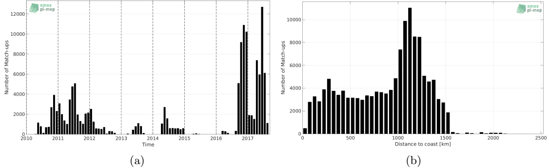
Figure 1: Number of match-ups between Surface drifters and SMOS-L3-CATDS-CECOS-IFREMER-V2-1DAY-0.5DEG SSS as a function of time (a) and as function of the distance to coast (b) over the Equatorial Ocean 10N-10S Pi-MEP region and for the full satellite product period.
