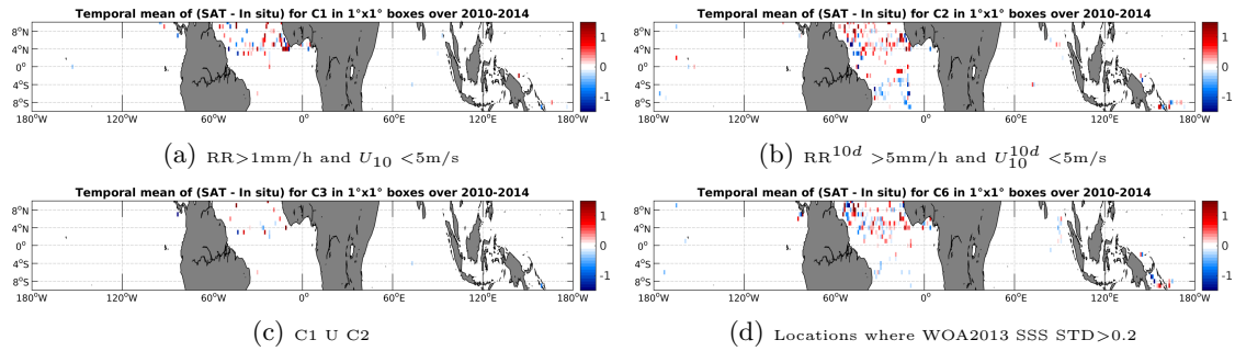
Figure 11: Temporal mean gridded over spatial boxes of size 1^\circ \times 1^\circ of \Delta SSS (SMOS-L3-CATDS-CECOS-IFREMER-V2-1DAY-0.5DEG - Surface drifters) for 4 different subdatasets corresponding to: RR > 1\text{mm/h} and U_{10} < 5\text{m/s} (a), RR^{10d} > 5\text{mm/h} and U_{10}^{10d} < 5\text{m/s} (b), C1 U C2 (c), Locations where WOA2013 SSS STD > 0.2 (d).
