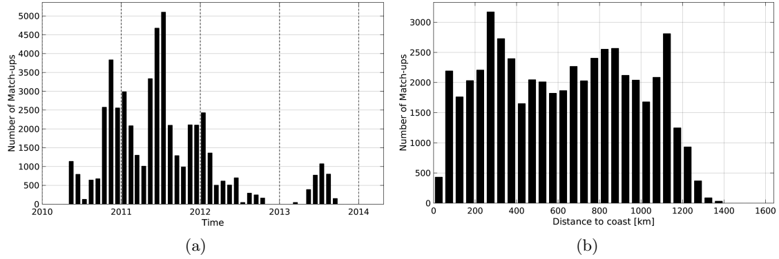
Figure 1: Number of match-ups between Surface drifters and SMOS-L3-CATDS-CECOS-IFREMER-V2-1DAY-0.5deg SSS as a function of time (a) and as function of the distance to coast (b) over the Equatorial Ocean 10N-10S Pi-MEP region and for the full satellite product period.
