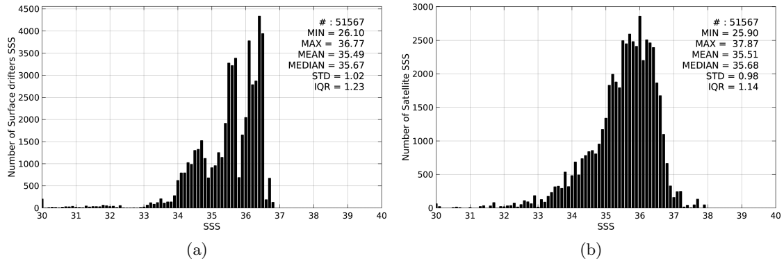
Figure 2: Histograms of SSS from Surface drifters (a) and SMOS-L3-CATDS-CECOS-IFREMER-V2-1DAY-0.5deg (b) considering all match-up pairs per bins of 0.1 over the Equatorial Ocean 10N-10S Pi-MEP region and for the full satellite product period.
