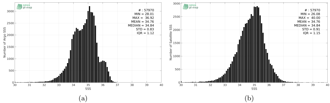
Figure 2: Histograms of SSS from Argo (a) and SMOS-L3-CATDS-CECOS-IFREMER-V2-1DAY-0.5DEG (b) considering all match-up pairs per bins of 0.1 over the Equatorial Ocean 10N-10S Pi-MEP region and for the full satellite product period.
