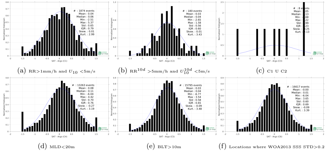
Figure 13: Normalized histogram of \Delta\text{SSS} (SMOS-L3-CATDS-CECOS-IFREMER-V2-1DAY-0.5DEG - Argo) for 6 different subdatasets corresponding to: \text{RR} > 1\text{mm/h} and U_{10} < 5\text{m/s} (a), \text{RR}^{10d} > 5\text{mm/h} and U_{10}^{10d} < 5\text{m/s} (b), C1 U C2 (c), \text{MLD} < 20\text{m} (d), \text{BLT} > 10\text{m} (e), Locations where WOA2013 SSS \text{STD} > 0.2 (f).
