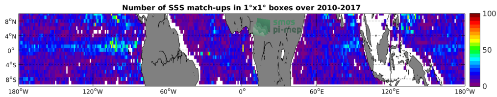
Figure 4: Number of SSS match-ups between Argo SSS and the SMOS-L3-CATDS-CECOS-IFREMER-V2-1DAY-0.5DEG SSS product for the Equatorial Ocean 10N-10S Pi-MEP region over 1^{\circ} \times 1^{\circ} boxes and for the full satellite product period.
