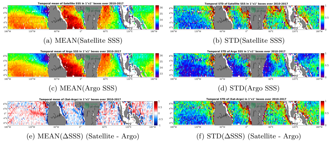
Figure 6: Temporal mean (left) and STD (right) of SSS from SMOS-L3-CATDS-CECOS-IFREMER-V2-1DAY-0.5DEG (top), Argo (middle), and of \Delta SSS (Satellite - Argo). Only match-up pairs are used to generate these maps.
