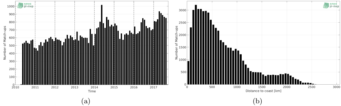
Figure 1: Number of match-ups between Argo and SMOS-L3-CATDS-CECOS-IFREMER-V2-1DAY-0.5DEG SSS as a function of time (a) and as function of the distance to coast (b) over the Equatorial Ocean 10N-10S Pi-MEP region and for the full satellite product period.
