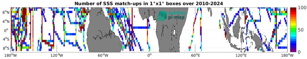
Figure 5: Number of SSS match-ups between TSG (SAMOS) SSS and the SMOS SSS L3 v335 - Monthly - 25 km (CATDS-CPDC) SSS product for the Equatorial Ocean 10N-10S Pi-MEP region over 1^\circ \times 1^\circ boxes and for the full satellite product period.
