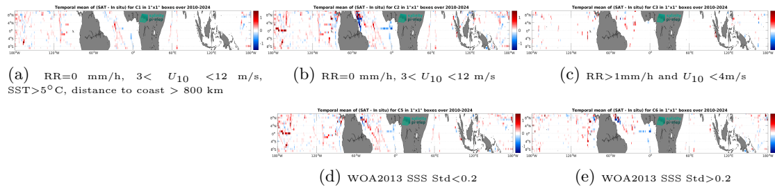
Figure 14: Temporal mean gridded over spatial boxes of size 1^\circ \times 1^\circ of \Delta SSS (SMOS SSS L3 v335 - Monthly - 25 km (CATDS-CPDC) - TSG (SAMOS)) for 5 different subdatasets corresponding to: RR=0 mm/h, 3 < U_{10} < 12 m/s, SST>5°C, distance to coast > 800 km (a), RR=0 mm/h, 3 < U_{10} < 12 m/s (b), RR>1mm/h and U_{10} < 4 m/s (c), WOA2013 SSS Std<0.2 (d), WOA2013 SSS Std>0.2 (e).
