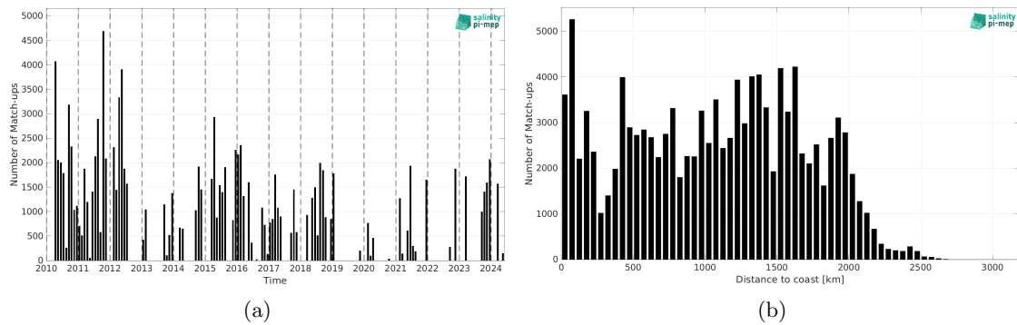
Figure 2: Number of match-ups between TSG (SAMOS) and SMOS SSS L3 v335 - Monthly - 25 km (CATDS-CPDC) SSS as a function of time (a) and as function of the distance to coast (b) over the Equatorial Ocean 10N-10S Pi-MEP region and for the full satellite product period.
