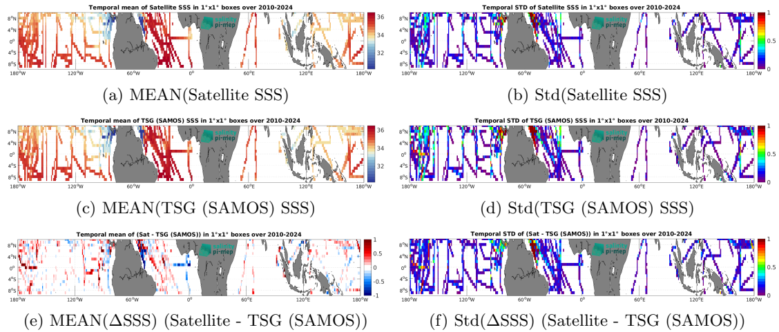
Figure 7: Temporal mean (left) and Std (right) of SSS from SMOS SSS L3 v335 - Monthly - 25 km (CATDS-CPDC) (top), TSG (SAMOS) (middle), and of \Delta SSS (Satellite - TSG (SAMOS)). Only match-up pairs are used to generate these maps.
