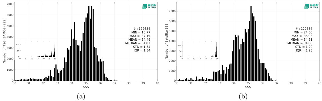
Figure 3: Histograms of SSS from TSG (SAMOS) (a) and SMOS SSS L3 v335 - Monthly - 25 km (CATDS-CPDC) (b) considering all match-up pairs per bins of 0.1 over the Equatorial Ocean 10N-10S Pi-MEP region and for the full satellite product period.
