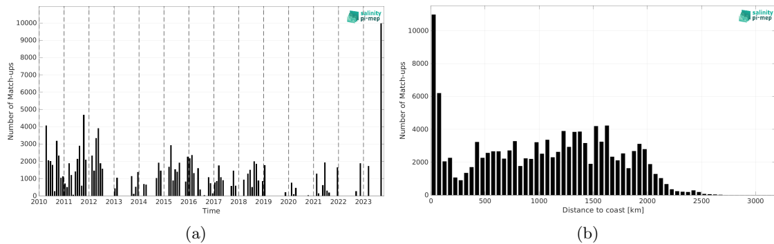
Figure 1: Number of match-ups between TSG (SAMOS) and SMOS SSS L3 v335 - Monthly - 25 km (CATDS-CPDC) SSS as a function of time (a) and as function of the distance to coast (b) over the Equatorial Ocean 10N-10S Pi-MEP region and for the full satellite product period.
