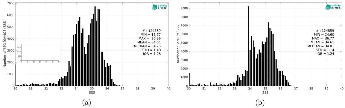
Figure 2: Histograms of SSS from TSG (SAMOS) (a) and SMOS SSS L3 v335 - Monthly - 25 km (CATDS-CPDC) (b) considering all match-up pairs per bins of 0.1 over the Equatorial Ocean 10N-10S Pi-MEP region and for the full satellite product period.
