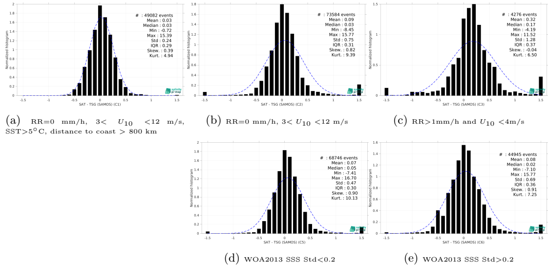
Figure 13: Normalized histogram of \Delta SSS (SMOS SSS L3 v335 - Monthly - 25 km (CATDS-CPDC) - TSG (SAMOS)) for 5 different subdatasets corresponding to: RR=0 mm/h, 3 < U_{10} < 12 m/s, SST >5^\circ\text{C} , distance to coast > 800 km (a), RR=0 mm/h, 3 < U_{10} < 12 m/s (b), RR >1 mm/h and U_{10} < 4 m/s (c), WOA2013 SSS Std <0.2 (d), WOA2013 SSS Std >0.2 (e).
