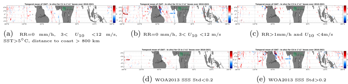
Figure 12: Temporal mean gridded over spatial boxes of size 1^\circ \times 1^\circ of \Delta SSS (SMOS SSS L3 v335 - Monthly - 25 km (CATDS-CPDC) - TSG (SAMOS)) for 5 different subdatasets corresponding to: RR=0 mm/h, 3 < U_{10} < 12 m/s, SST >5^\circ\text{C} , distance to coast > 800 km (a), RR=0 mm/h, 3 < U_{10} < 12 m/s (b), RR >1 mm/h and U_{10} < 4 m/s (c), WOA2013 SSS Std <0.2 (d), WOA2013 SSS Std >0.2 (e).
