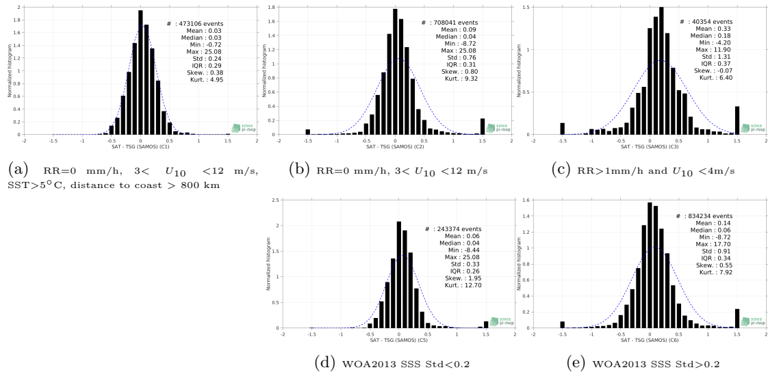
Figure 13: Normalized histogram of \Delta SSS (SMOS SSS L3 v335 - Monthly - 25 km (CATDS-CPDC) - TSG (SAMOS)) for 5 different subdatasets corresponding to: RR=0 mm/h, 3 < U_{10} < 12 m/s, SST >5^\circ\text{C} , distance to coast > 800 km (a), RR=0 mm/h, 3 < U_{10} < 12 m/s (b), RR >1 mm/h and U_{10} < 4 m/s (c), WOA2013 SSS Std <0.2 (d), WOA2013 SSS Std >0.2 (e).
