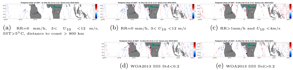
Figure 14: Temporal mean gridded over spatial boxes of size 1^\circ \times 1^\circ of \Delta\text{SSS} (SMOS SSS L3 v335 - Monthly - 25 km (CATDS-CPDC) - TSG (LEGOS-DM)) for 5 different subdatasets corresponding to:RR=0 mm/h, 3 < U_{10} < 12 m/s, SST>5°C, distance to coast > 800 km (a), RR=0 mm/h, 3 < U_{10} < 12 m/s (b), RR>1mm/h and U_{10} < 4 m/s (c), WOA2013 SSS Std<0.2 (d), WOA2013 SSS Std>0.2 (e).
