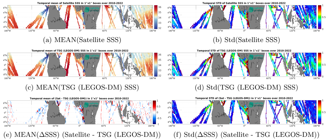
Figure 7: Temporal mean (left) and Std (right) of SSS from SMOS SSS L3 v335 - Monthly - 25 km (CATDS-CPDC) (top), TSG (LEGOS-DM) (middle), and of \Delta SSS (Satellite - TSG (LEGOS-DM)). Only match-up pairs are used to generate these maps.
