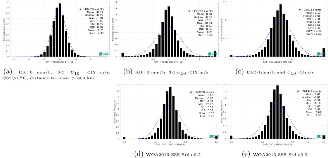
Figure 15: Normalized histogram of \Delta\text{SSS} (SMOS SSS L3 v335 - Monthly - 25 km (CATDS-CPDC) - TSG (LEGOS-DM)) for 5 different subdatasets corresponding to: RR=0 mm/h, 3 < U_{10} < 12 m/s, SST>5°C, distance to coast > 800 km (a), RR=0 mm/h, 3 < U_{10} < 12 m/s (b), RR>1mm/h and U_{10} < 4 m/s (c), WOA2013 SSS Std<0.2 (d), WOA2013 SSS Std>0.2 (e).
