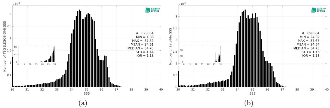
Figure 3: Histograms of SSS from TSG (LEGOS-DM) (a) and SMOS SSS L3 v335 - Monthly - 25 km (CATDS-CPDC) (b) considering all match-up pairs per bins of 0.1 over the Equatorial Ocean 10N-10S Pi-MEP region and for the full satellite product period.
