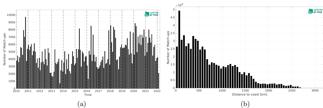
Figure 2: Number of match-ups between TSG (LEGOS-DM) and SMOS SSS L3 v335 - Monthly - 25 km (CATDS-CPDC) SSS as a function of time (a) and as function of the distance to coast (b) over the Equatorial Ocean 10N-10S Pi-MEP region and for the full satellite product period.
