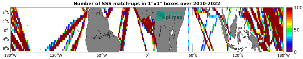
Figure 5: Number of SSS match-ups between TSG (LEGOS-DM) SSS and the SMOS SSS L3 v335 - Monthly - 25 km (CATDS-CPDC) SSS product for the Equatorial Ocean 10N-10S Pi-MEP region over 1^\circ \times 1^\circ boxes and for the full satellite product period.
