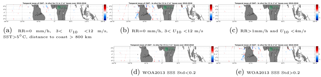
Figure 12: Temporal mean gridded over spatial boxes of size 1^\circ \times 1^\circ of \Delta SSS (SMOS SSS L3 v335 - Monthly - 25 km (CATDS-CPDC) - TSG (GOSUD-Sailing-ship)) for 5 different subdatasets corresponding to:RR=0 mm/h, 3 < U_{10} < 12 m/s, SST > 5^\circ\text{C} , distance to coast > 800 km (a), RR=0 mm/h, 3 < U_{10} < 12 m/s (b), RR > 1 mm/h and U_{10} < 4 m/s (c), WOA2013 SSS Std < 0.2 (d), WOA2013 SSS Std > 0.2 (e).
