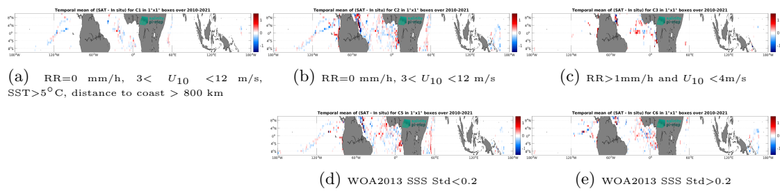
Figure 12: Temporal mean gridded over spatial boxes of size 1^\circ \times 1^\circ of \Delta\text{SSS} (SMOS SSS L3 v335 - Monthly - 25 km (CATDS-CPDC) - TSG (GOSUD-Research-vessel)) for 5 different subdatasets corresponding to:RR=0 mm/h, 3 < U_{10} < 12 m/s, SST > 5°C, distance to coast > 800 km (a), RR=0 mm/h, 3 < U_{10} < 12 m/s (b), RR > 1mm/h and U_{10} < 4 m/s (c), WOA2013 SSS Std < 0.2 (d), WOA2013 SSS Std > 0.2 (e).
