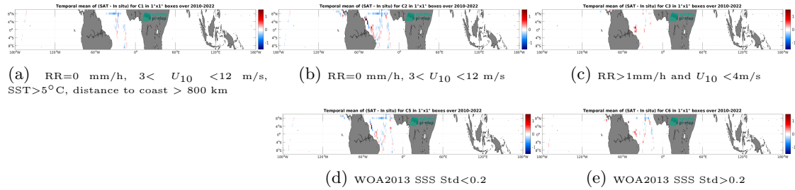
Figure 14: Temporal mean gridded over spatial boxes of size 1^\circ \times 1^\circ of \Delta SSS (SMOS SSS L3 v335 - Monthly - 25 km (CATDS-CPDC) - TSG (CSIC-UTM)) for 5 different subdatasets corresponding to: RR=0 mm/h, 3 < U_{10} < 12 m/s, SST>5°C, distance to coast > 800 km (a), RR=0 mm/h, 3 < U_{10} < 12 m/s (b), RR>1mm/h and U_{10} < 4 m/s (c), WOA2013 SSS Std<0.2 (d), WOA2013 SSS Std>0.2 (e).
