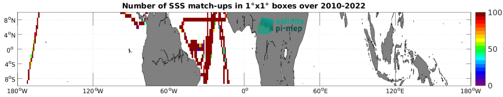
Figure 5: Number of SSS match-ups between TSG (CSIC-UTM) SSS and the SMOS SSS L3 v335 - Monthly - 25 km (CATDS-CPDC) SSS product for the Equatorial Ocean 10N-10S Pi-MEP region over 1^\circ \times 1^\circ boxes and for the full satellite product period.
