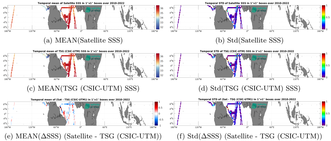
Figure 7: Temporal mean (left) and Std (right) of SSS from SMOS SSS L3 v335 - Monthly - 25 km (CATDS-CPDC) (top), TSG (CSIC-UTM) (middle), and of \Delta SSS (Satellite - TSG (CSIC-UTM)). Only match-up pairs are used to generate these maps.
