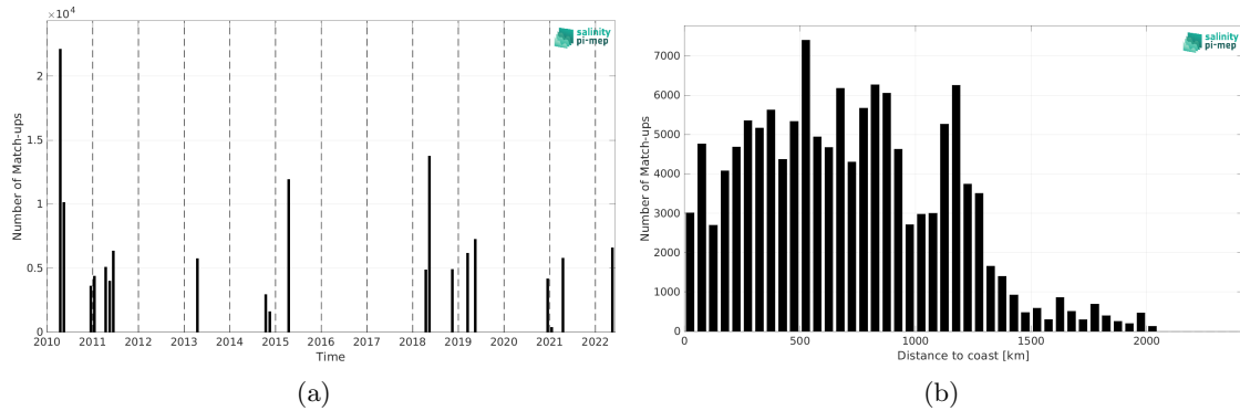
Figure 2: Number of match-ups between TSG (CSIC-UTM) and SMOS SSS L3 v335 - Monthly - 25 km (CATDS-CPDC) SSS as a function of time (a) and as function of the distance to coast (b) over the Equatorial Ocean 10N-10S Pi-MEP region and for the full satellite product period.
