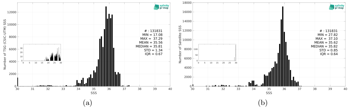
Figure 3: Histograms of SSS from TSG (CSIC-UTM) (a) and SMOS SSS L3 v335 - Monthly - 25 km (CATDS-CPDC) (b) considering all match-up pairs per bins of 0.1 over the Equatorial Ocean 10N-10S Pi-MEP region and for the full satellite product period.
