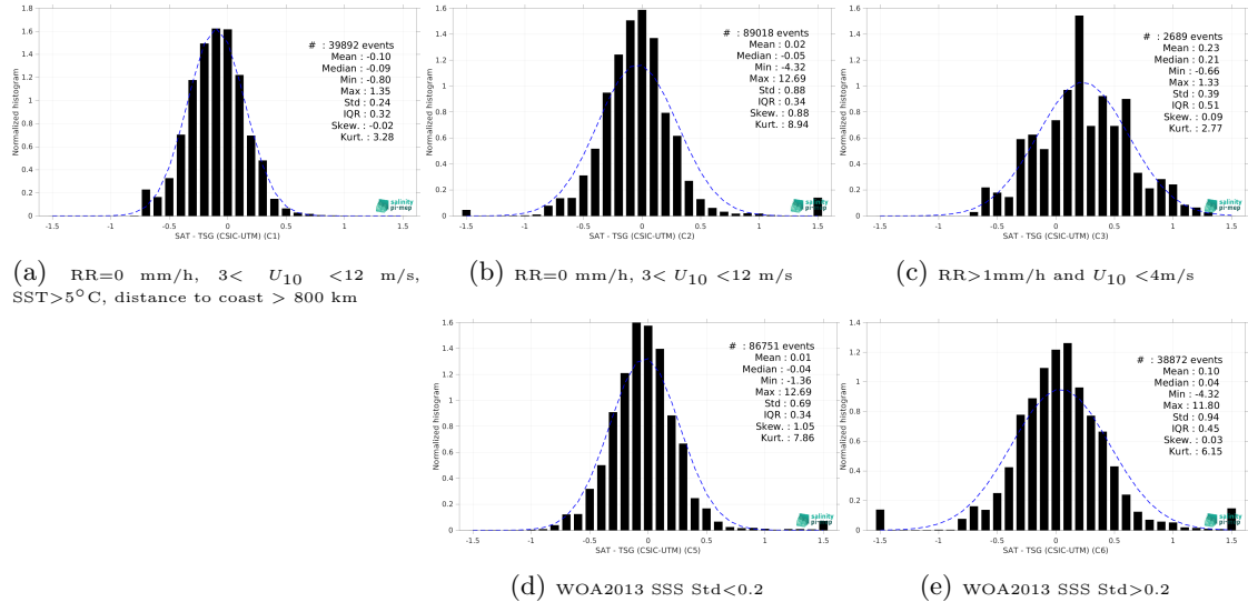
Figure 15: Normalized histogram of \Delta SSS (SMOS SSS L3 v335 - Monthly - 25 km (CATDS-CPDC) - TSG (CSIC-UTM)) for 5 different subdatasets corresponding to: RR=0 mm/h, 3 < U_{10} < 12 m/s, SST>5°C, distance to coast > 800 km (a), RR=0 mm/h, 3 < U_{10} < 12 m/s (b), RR>1mm/h and U_{10} < 4 m/s (c), WOA2013 SSS Std<0.2 (d), WOA2013 SSS Std>0.2 (e).
