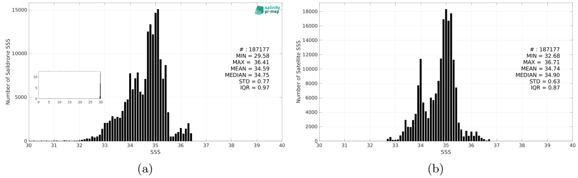
Figure 3: Histograms of SSS from Saildrone (a) and SMOS SSS L3 v335 - Monthly - 25 km (CATDS-CPDC) (b) considering all match-up pairs per bins of 0.1 over the Equatorial Ocean 10N-10S Pi-MEP region and for the full satellite product period.
