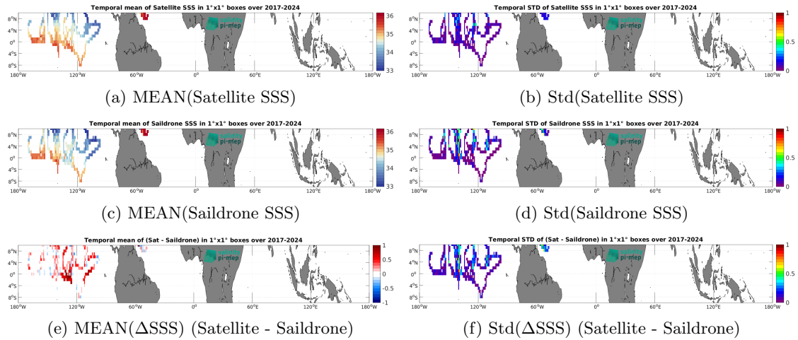
Figure 7: Temporal mean (left) and Std (right) of SSS from SMOS SSS L3 v335 - Monthly - 25 km (CATDS-CPDC) (top), Saildrone (middle), and of \Delta SSS (Satellite - Saildrone). Only match-up pairs are used to generate these maps.
