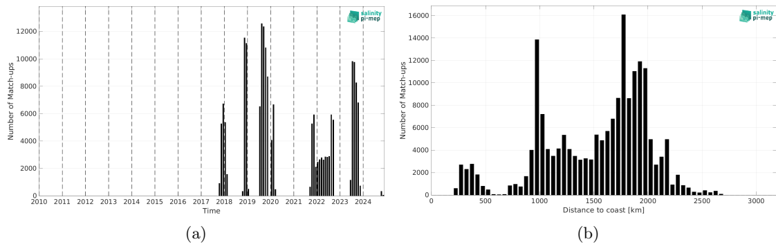
Figure 2: Number of match-ups between Saildrone and SMOS SSS L3 v335 - Monthly - 25 km (CATDS-CPDC) SSS as a function of time (a) and as function of the distance to coast (b) over the Equatorial Ocean 10N-10S Pi-MEP region and for the full satellite product period.
