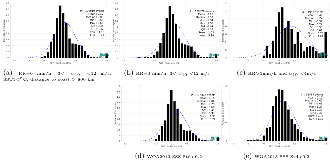
Figure 15: Normalized histogram of \Delta SSS (SMOS SSS L3 v335 - Monthly - 25 km (CATDS-CPDC) - Sailydrone) for 5 different subdatasets corresponding to: RR=0 mm/h, 3 < U_{10} < 12 m/s, SST>5°C, distance to coast > 800 km (a), RR=0 mm/h, 3 < U_{10} < 12 m/s (b), RR>1mm/h and U_{10} < 4 m/s (c), WOA2013 SSS Std<0.2 (d), WOA2013 SSS Std>0.2 (e).
