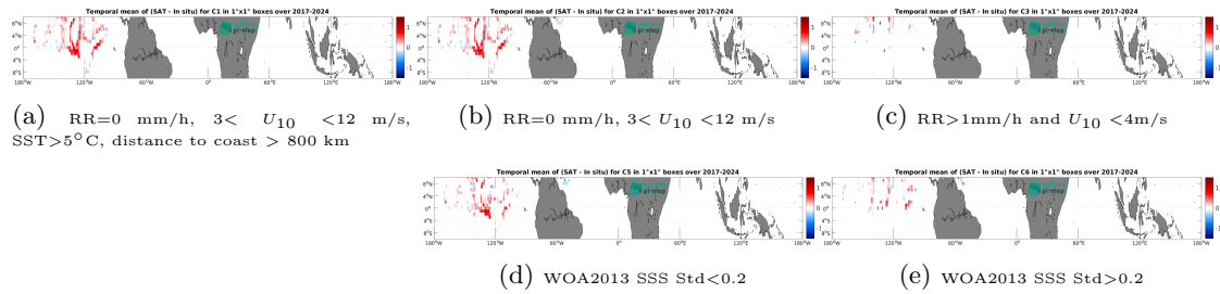
Figure 14: Temporal mean gridded over spatial boxes of size 1^\circ \times 1^\circ of \Delta SSS (SMOS SSS L3 v335 - Monthly - 25 km (CATDS-CPDC) - Sailydrone) for 5 different subdatasets corresponding to: RR=0 mm/h, 3 < U_{10} < 12 m/s, SST>5°C, distance to coast > 800 km (a), RR=0 mm/h, 3 < U_{10} < 12 m/s (b), RR>1mm/h and U_{10} < 4 m/s (c), WOA2013 SSS Std<0.2 (d), WOA2013 SSS Std>0.2 (e).
