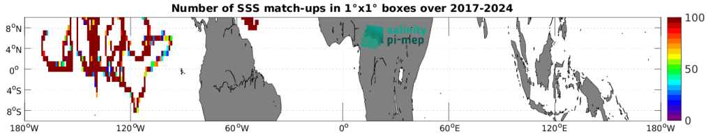
Figure 5: Number of SSS match-ups between Saildrone SSS and the SMOS SSS L3 v335 - Monthly - 25 km (CATDS-CPDC) SSS product for the Equatorial Ocean 10N-10S Pi-MEP region over 1^\circ \times 1^\circ boxes and for the full satellite product period.
