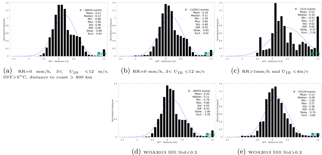
Figure 15: Normalized histogram of \Delta SSS (SMOS SSS L3 v335 - Monthly - 25 km (CATDS-CPDC) - Saildrone) for 5 different subdatasets corresponding to: RR=0 mm/h, 3 < U_{10} < 12 m/s, SST >5^\circ\text{C} , distance to coast > 800 km (a), RR=0 mm/h, 3 < U_{10} < 12 m/s (b), RR >1 mm/h and U_{10} < 4 m/s (c), WOA2013 SSS Std <0.2 (d), WOA2013 SSS Std >0.2 (e).
