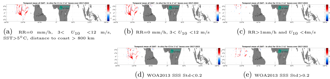
Figure 14: Temporal mean gridded over spatial boxes of size 1^\circ \times 1^\circ of \Delta SSS (SMOS SSS L3 v335 - Monthly - 25 km (CATDS-CPDC) - Saildrone) for 5 different subdatasets corresponding to: RR=0 mm/h, 3 < U_{10} < 12 m/s, SST >5^\circ\text{C} , distance to coast > 800 km (a), RR=0 mm/h, 3 < U_{10} < 12 m/s (b), RR >1 mm/h and U_{10} < 4 m/s (c), WOA2013 SSS Std <0.2 (d), WOA2013 SSS Std >0.2 (e).
