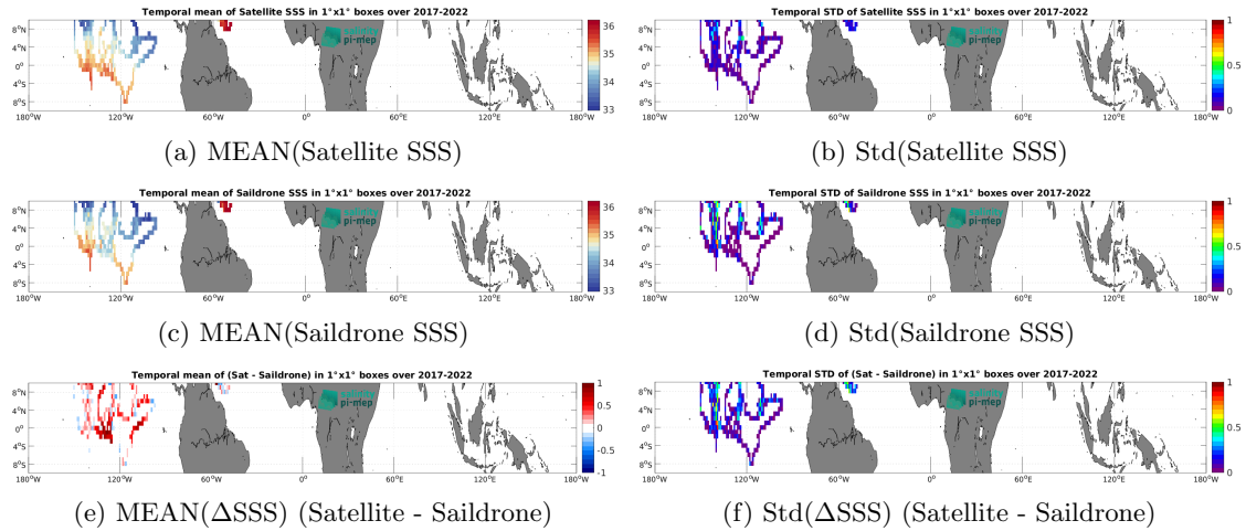
Figure 6: Temporal mean (left) and Std (right) of SSS from SMOS SSS L3 v335 - Monthly - 25 km (CATDS-CPDC) (top), Saildrone (middle), and of \Delta SSS (Satellite - Saildrone). Only match-up pairs are used to generate these maps.
