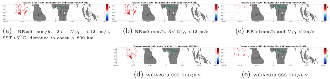
Figure 12: Temporal mean gridded over spatial boxes of size 1^\circ \times 1^\circ of \Delta SSS (SMOS SSS L3 v335 - Monthly - 25 km (CATDS-CPDC) - Saldrone) for 5 different subdatasets corresponding to:RR=0 mm/h, 3 < U_{10} < 12 m/s, SST>5°C, distance to coast > 800 km (a), RR=0 mm/h, 3 < U_{10} < 12 m/s (b), RR>1mm/h and U_{10} < 4 m/s (c), WOA2013 SSS Std<0.2 (d), WOA2013 SSS Std>0.2 (e).
