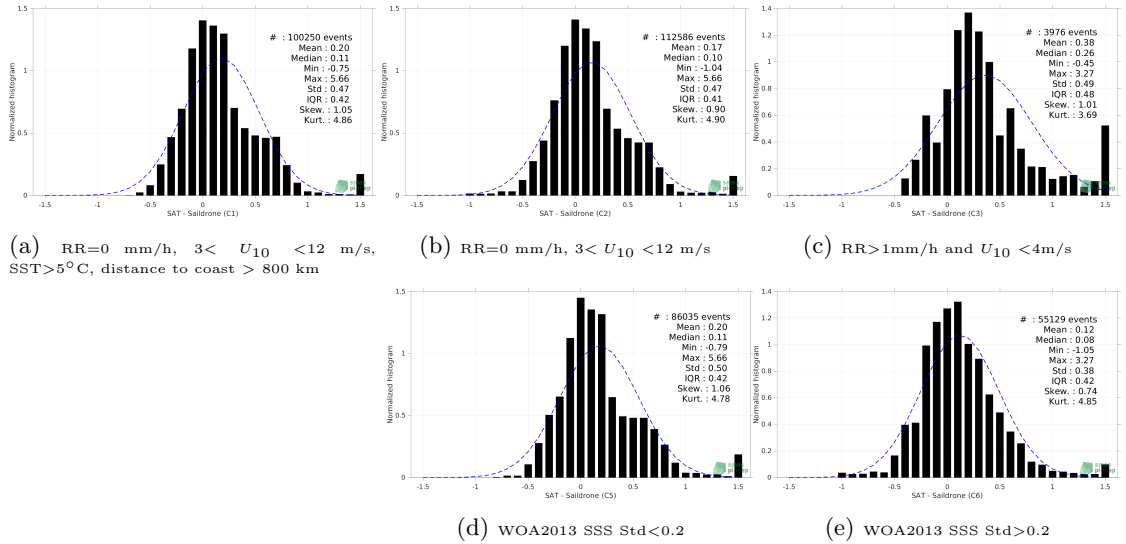
Figure 13: Normalized histogram of \Delta SSS (SMOS SSS L3 v335 - Monthly - 25 km (CATDS-CPDC) - Saldrone) for 5 different subdatasets corresponding to: RR=0 mm/h, 3 < U_{10} < 12 m/s, SST>5°C, distance to coast > 800 km (a), RR=0 mm/h, 3 < U_{10} < 12 m/s (b), RR>1mm/h and U_{10} < 4 m/s (c), WOA2013 SSS Std<0.2 (d), WOA2013 SSS Std>0.2 (e).
