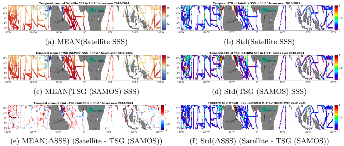
Figure 7: Temporal mean (left) and Std (right) of SSS from SMOS SSS L3 v335 - 10 Days - 25 km (CATDS-CPDC) (top), TSG (SAMOS) (middle), and of \Delta SSS (Satellite - TSG (SAMOS)). Only match-up pairs are used to generate these maps.
