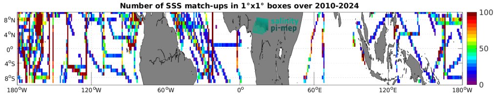
Figure 5: Number of SSS match-ups between TSG (SAMOS) SSS and the SMOS SSS L3 v335 - 10 Days - 25 km (CATDS-CPDC) SSS product for the Equatorial Ocean 10N-10S Pi-MEP region over 1^\circ \times 1^\circ boxes and for the full satellite product period.
