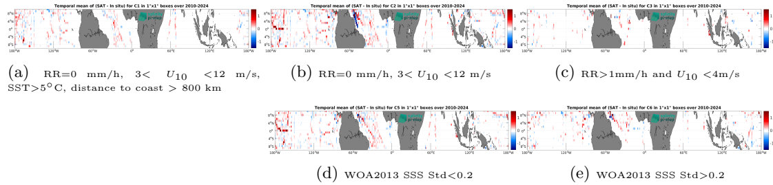
Figure 14: Temporal mean gridded over spatial boxes of size 1^\circ \times 1^\circ of \Delta SSS (SMOS SSS L3 v335 - 10 Days - 25 km (CATDS-CPDC) - TSG (SAMOS)) for 5 different subdatasets corresponding to: RR=0 mm/h, 3 < U_{10} < 12 m/s, SST>5°C, distance to coast > 800 km (a), RR=0 mm/h, 3 < U_{10} < 12 m/s (b), RR>1mm/h and U_{10} < 4 m/s (c), WOA2013 SSS Std<0.2 (d), WOA2013 SSS Std>0.2 (e).
