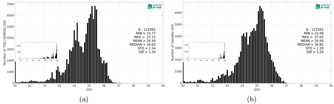
Figure 3: Histograms of SSS from TSG (SAMOS) (a) and SMOS SSS L3 v335 - 10 Days - 25 km (CATDS-CPDC) (b) considering all match-up pairs per bins of 0.1 over the Equatorial Ocean 10N-10S Pi-MEP region and for the full satellite product period.
