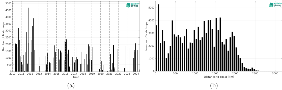
Figure 2: Number of match-ups between TSG (SAMOS) and SMOS SSS L3 v335 - 10 Days - 25 km (CATDS-CPDC) SSS as a function of time (a) and as function of the distance to coast (b) over the Equatorial Ocean 10N-10S Pi-MEP region and for the full satellite product period.
