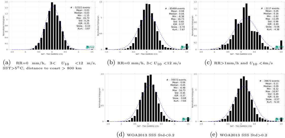
Figure 15: Normalized histogram of \Delta SSS (SMOS SSS L3 v335 - 10 Days - 25 km (CATDS-CPDC) - TSG (SAMOS)) for 5 different subdatasets corresponding to: RR=0 mm/h, 3 < U_{10} < 12 m/s, SST>5°C, distance to coast > 800 km (a), RR=0 mm/h, 3 < U_{10} < 12 m/s (b), RR>1mm/h and U_{10} < 4 m/s (c), WOA2013 SSS Std<0.2 (d), WOA2013 SSS Std>0.2 (e).
