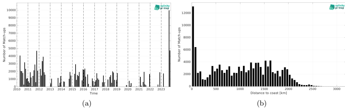
Figure 1: Number of match-ups between TSG (SAMOS) and SMOS SSS L3 v335 - 10 Days - 25 km (CATDS-CPDC) SSS as a function of time (a) and as function of the distance to coast (b) over the Equatorial Ocean 10N-10S Pi-MEP region and for the full satellite product period.
