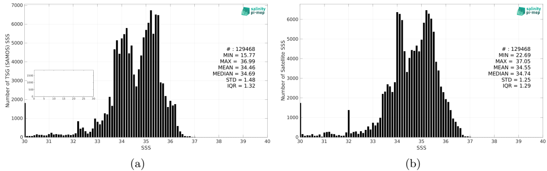
Figure 2: Histograms of SSS from TSG (SAMOS) (a) and SMOS SSS L3 v335 - 10 Days - 25 km (CATDS-CPDC) (b) considering all match-up pairs per bins of 0.1 over the Equatorial Ocean 10N-10S Pi-MEP region and for the full satellite product period.
