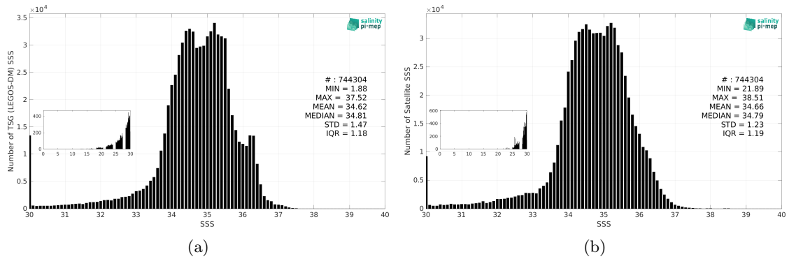
Figure 3: Histograms of SSS from TSG (LEGOS-DM) (a) and SMOS SSS L3 v335 - 10 Days - 25 km (CATDS-CPDC) (b) considering all match-up pairs per bins of 0.1 over the Equatorial Ocean 10N-10S Pi-MEP region and for the full satellite product period.
