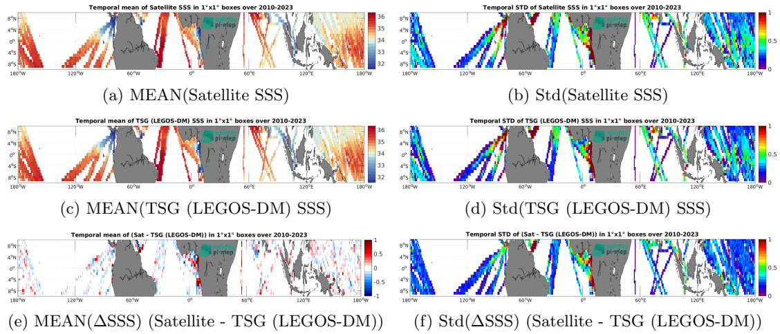
Figure 7: Temporal mean (left) and Std (right) of SSS from SMOS SSS L3 v335 - 10 Days - 25 km (CATDS-CPDC) (top), TSG (LEGOS-DM) (middle), and of \Delta SSS (Satellite - TSG (LEGOS-DM)). Only match-up pairs are used to generate these maps.
