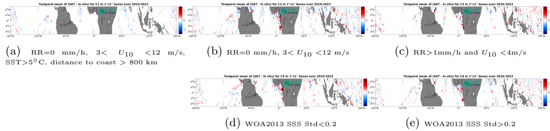
Figure 14: Temporal mean gridded over spatial boxes of size 1^\circ \times 1^\circ of \Delta\text{SSS} (SMOS SSS L3 v335 - 10 Days - 25 km (CATDS-CPDC) - TSG (LEGOS-DM)) for 5 different subdatasets corresponding to: RR=0 mm/h, 3 < U_{10} < 12 m/s, SST>5°C, distance to coast > 800 km (a), RR=0 mm/h, 3 < U_{10} < 12 m/s (b), RR>1mm/h and U_{10} < 4 m/s (c), WOA2013 SSS Std<0.2 (d), WOA2013 SSS Std>0.2 (e).
