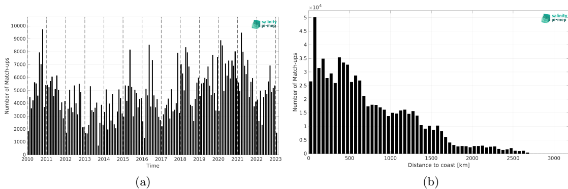
Figure 2: Number of match-ups between TSG (LEGOS-DM) and SMOS SSS L3 v335 - 10 Days - 25 km (CATDS-CPDC) SSS as a function of time (a) and as function of the distance to coast (b) over the Equatorial Ocean 10N-10S Pi-MEP region and for the full satellite product period.
