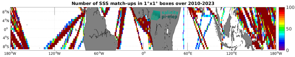
Figure 5: Number of SSS match-ups between TSG (LEGOS-DM) SSS and the SMOS SSS L3 v335 - 10 Days - 25 km (CATDS-CPDC) SSS product for the Equatorial Ocean 10N-10S Pi-MEP region over 1^\circ \times 1^\circ boxes and for the full satellite product period.
