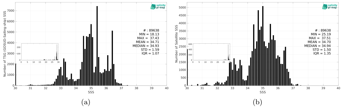
Figure 3: Histograms of SSS from TSG (GOSUD-Sailing-ship) (a) and SMOS SSS L3 v335 - 10 Days - 25 km (CATDS-CPDC) (b) considering all match-up pairs per bins of 0.1 over the Equatorial Ocean 10N-10S Pi-MEP region and for the full satellite product period.
