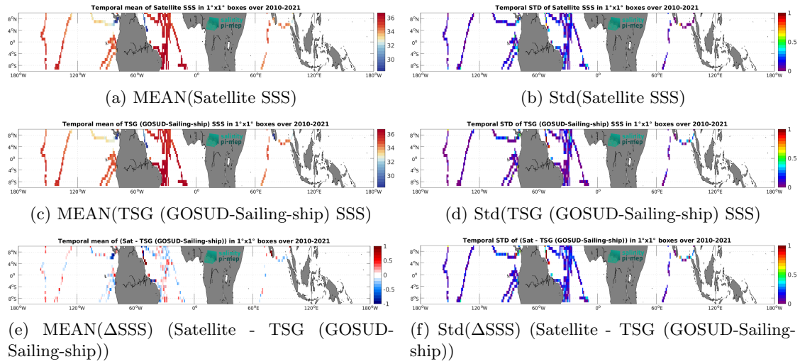
Figure 7: Temporal mean (left) and Std (right) of SSS from SMOS SSS L3 v335 - 10 Days - 25 km (CATDS-CPDC) (top), TSG (GOSUD-Sailing-ship) (middle), and of \Delta SSS (Satellite - TSG (GOSUD-Sailing-ship)). Only match-up pairs are used to generate these maps.
