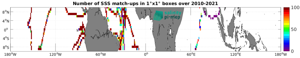
Figure 5: Number of SSS match-ups between TSG (GOSUD-Sailing-ship) SSS and the SMOS SSS L3 v335 - 10 Days - 25 km (CATDS-CPDC) SSS product for the Equatorial Ocean 10N-10S Pi-MEP region over 1^\circ \times 1^\circ boxes and for the full satellite product period.
