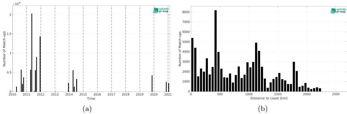
Figure 2: Number of match-ups between TSG (GOSUD-Sailing-ship) and SMOS SSS L3 v335 - 10 Days - 25 km (CATDS-CPDC) SSS as a function of time (a) and as function of the distance to coast (b) over the Equatorial Ocean 10N-10S Pi-MEP region and for the full satellite product period.
