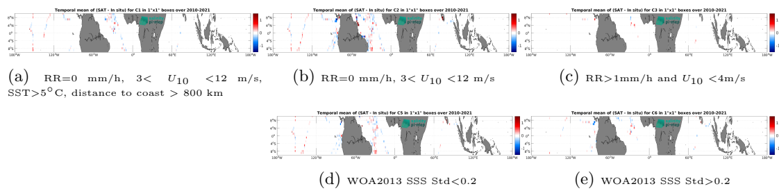
Figure 14: Temporal mean gridded over spatial boxes of size 1^\circ \times 1^\circ of \Delta\text{SSS} (SMOS SSS L3 v335 - 10 Days - 25 km (CATDS-CPDC) - TSG (GOSUD-Sailing-ship)) for 5 different subdatasets corresponding to:RR=0 mm/h, 3 < U_{10} < 12 m/s, SST > 5°C, distance to coast > 800 km (a), RR=0 mm/h, 3 < U_{10} < 12 m/s (b), RR > 1mm/h and U_{10} < 4 m/s (c), WOA2013 SSS Std < 0.2 (d), WOA2013 SSS Std > 0.2 (e).
