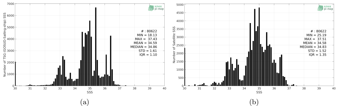
Figure 2: Histograms of SSS from TSG (GOSUD-Sailing-ship) (a) and SMOS SSS L3 v335 - 10 Days - 25 km (CATDS-CPDC) (b) considering all match-up pairs per bins of 0.1 over the Equatorial Ocean 10N-10S Pi-MEP region and for the full satellite product period.
