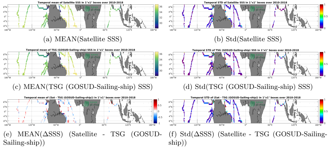
Figure 6: Temporal mean (left) and Std (right) of SSS from SMOS SSS L3 v335 - 10 Days - 25 km (CATDS-CPDC) (top), TSG (GOSUD-Sailing-ship) (middle), and of \Delta SSS (Satellite - TSG (GOSUD-Sailing-ship)). Only match-up pairs are used to generate these maps.
