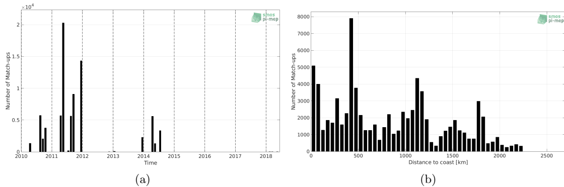
Figure 1: Number of match-ups between TSG (GOSUD-Sailing-ship) and SMOS SSS L3 v335 - 10 Days - 25 km (CATDS-CPDC) SSS as a function of time (a) and as function of the distance to coast (b) over the Equatorial Ocean 10N-10S Pi-MEP region and for the full satellite product period.
