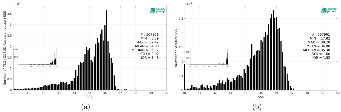
Figure 3: Histograms of SSS from TSG (GOSUD-Research-vessel) (a) and SMOS SSS L3 v335 - 10 Days - 25 km (CATDS-CPDC) (b) considering all match-up pairs per bins of 0.1 over the Equatorial Ocean 10N-10S Pi-MEP region and for the full satellite product period.
