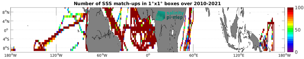
Figure 5: Number of SSS match-ups between TSG (GOSUD-Research-vessel) SSS and the SMOS SSS L3 v335 - 10 Days - 25 km (CATDS-CPDC) SSS product for the Equatorial Ocean 10N-10S Pi-MEP region over 1^\circ \times 1^\circ boxes and for the full satellite product period.
