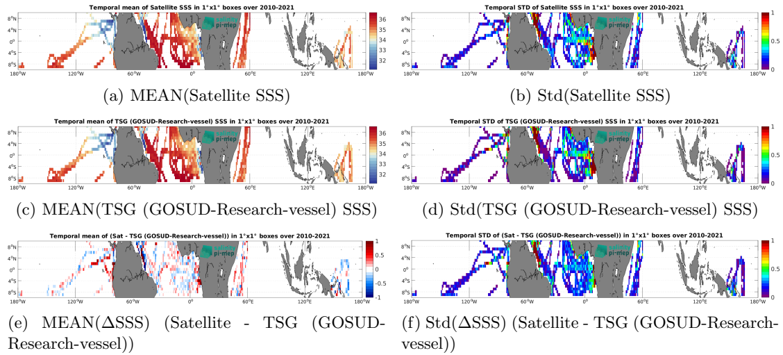
Figure 7: Temporal mean (left) and Std (right) of SSS from SMOS SSS L3 v335 - 10 Days - 25 km (CATDS-CPDC) (top), TSG (GOSUD-Research-vessel) (middle), and of \Delta SSS (Satellite - TSG (GOSUD-Research-vessel)). Only match-up pairs are used to generate these maps.
