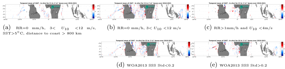
Figure 12: Temporal mean gridded over spatial boxes of size 1^\circ \times 1^\circ of \Delta\text{SSS} (SMOS SSS L3 v335 - 10 Days - 25 km (CATDS-CPDC) - TSG (GOSUD-Research-vessel)) for 5 different subdatasets corresponding to:RR=0 mm/h, 3 < U_{10} < 12 m/s, SST > 5°C, distance to coast > 800 km (a), RR=0 mm/h, 3 < U_{10} < 12 m/s (b), RR > 1mm/h and U_{10} < 4 m/s (c), WOA2013 SSS Std < 0.2 (d), WOA2013 SSS Std > 0.2 (e).
