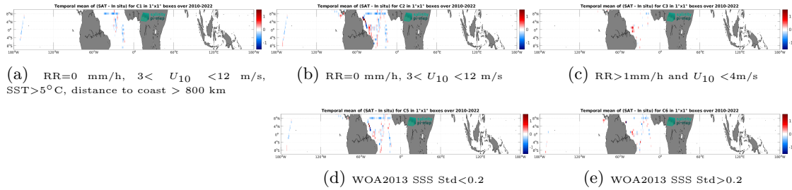
Figure 14: Temporal mean gridded over spatial boxes of size 1^\circ \times 1^\circ of \Delta SSS (SMOS SSS L3 v335 - 10 Days - 25 km (CATDS-CPDC) - TSG (CSIC-UTM)) for 5 different subdatasets corresponding to: RR=0 mm/h, 3 < U_{10} < 12 m/s, SST >5^\circ C, distance to coast > 800 km (a), RR=0 mm/h, 3 < U_{10} < 12 m/s (b), RR >1 mm/h and U_{10} < 4 m/s (c), WOA2013 SSS Std <0.2 (d), WOA2013 SSS Std >0.2 (e).
