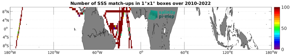
Figure 5: Number of SSS match-ups between TSG (CSIC-UTM) SSS and the SMOS SSS L3 v335 - 10 Days - 25 km (CATDS-CPDC) SSS product for the Equatorial Ocean 10N-10S Pi-MEP region over 1^\circ \times 1^\circ boxes and for the full satellite product period.
