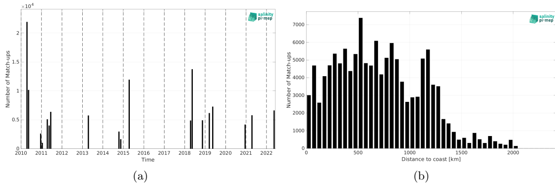
Figure 2: Number of match-ups between TSG (CSIC-UTM) and SMOS SSS L3 v335 - 10 Days - 25 km (CATDS-CPDC) SSS as a function of time (a) and as function of the distance to coast (b) over the Equatorial Ocean 10N-10S Pi-MEP region and for the full satellite product period.
