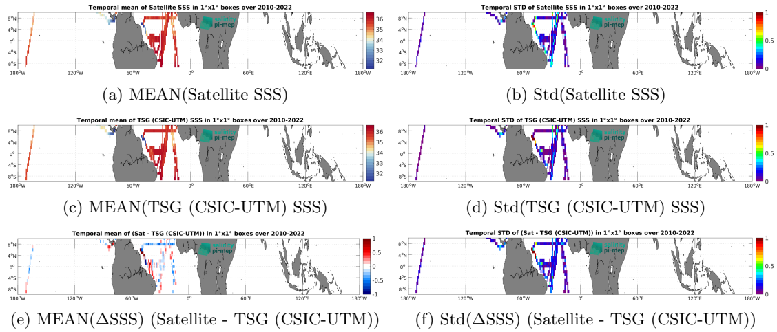
Figure 7: Temporal mean (left) and Std (right) of SSS from SMOS SSS L3 v335 - 10 Days - 25 km (CATDS-CPDC) (top), TSG (CSIC-UTM) (middle), and of \Delta SSS (Satellite - TSG (CSIC-UTM)). Only match-up pairs are used to generate these maps.
