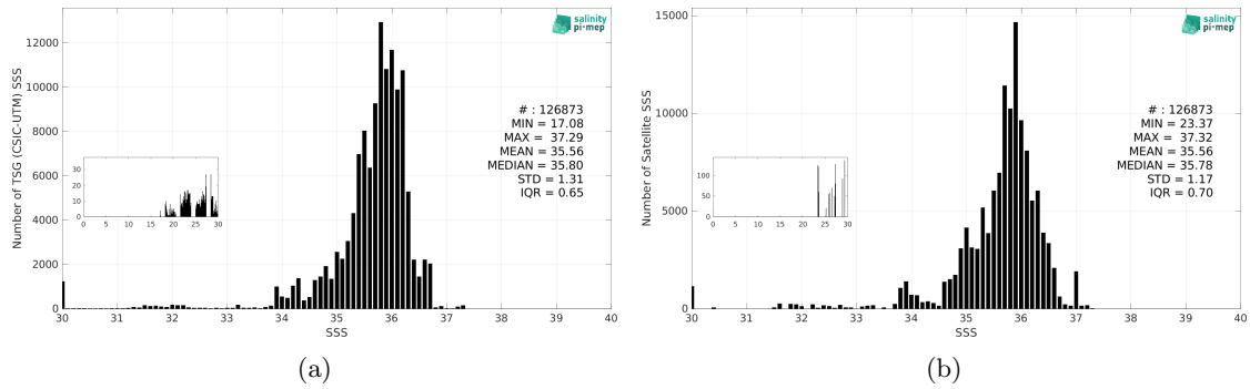
Figure 3: Histograms of SSS from TSG (CSIC-UTM) (a) and SMOS SSS L3 v335 - 10 Days - 25 km (CATDS-CPDC) (b) considering all match-up pairs per bins of 0.1 over the Equatorial Ocean 10N-10S Pi-MEP region and for the full satellite product period.
