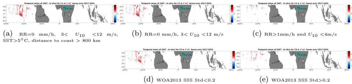
Figure 14: Temporal mean gridded over spatial boxes of size 1^\circ \times 1^\circ of \Delta SSS (SMOS SSS L3 v335 - 10 Days - 25 km (CATDS-CPDC) - Sailydrone) for 5 different subdatasets corresponding to: RR=0 mm/h, 3 < U_{10} < 12 m/s, SST>5°C, distance to coast > 800 km (a), RR=0 mm/h, 3 < U_{10} < 12 m/s (b), RR>1mm/h and U_{10} < 4 m/s (c), WOA2013 SSS Std<0.2 (d), WOA2013 SSS Std>0.2 (e).
