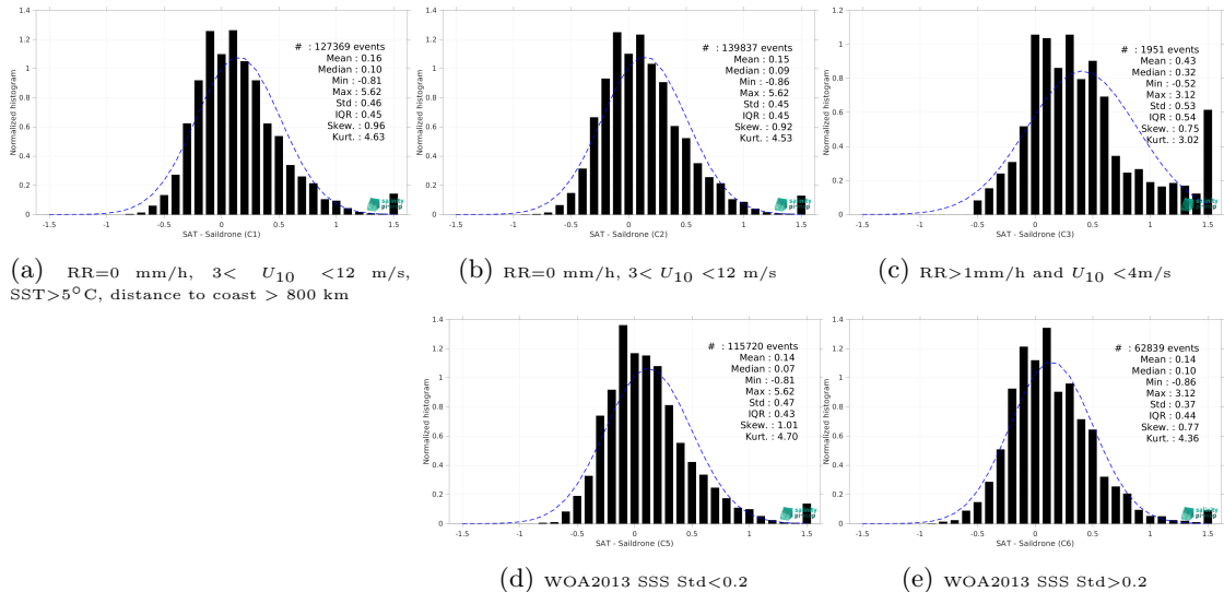
Figure 15: Normalized histogram of \Delta SSS (SMOS SSS L3 v335 - 10 Days - 25 km (CATDS-CPDC) - Sailydrone) for 5 different subdatasets corresponding to: RR=0 mm/h, 3 < U_{10} < 12 m/s, SST>5°C, distance to coast > 800 km (a), RR=0 mm/h, 3 < U_{10} < 12 m/s (b), RR>1mm/h and U_{10} < 4 m/s (c), WOA2013 SSS Std<0.2 (d), WOA2013 SSS Std>0.2 (e).
