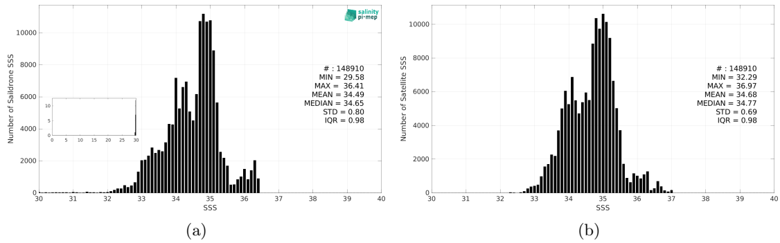
Figure 3: Histograms of SSS from Saildrone (a) and SMOS SSS L3 v335 - 10 Days - 25 km (CATDS-CPDC) (b) considering all match-up pairs per bins of 0.1 over the Equatorial Ocean 10N-10S Pi-MEP region and for the full satellite product period.
