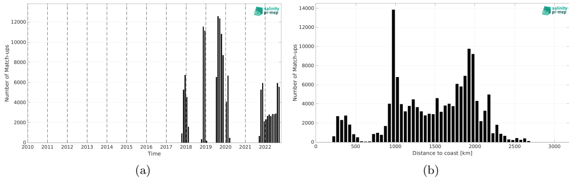
Figure 2: Number of match-ups between Saildrone and SMOS SSS L3 v335 - 10 Days - 25 km (CATDS-CPDC) SSS as a function of time (a) and as function of the distance to coast (b) over the Equatorial Ocean 10N-10S Pi-MEP region and for the full satellite product period.
