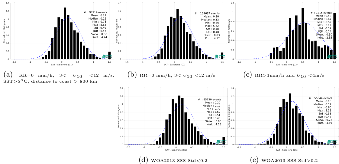
Figure 15: Normalized histogram of \Delta SSS (SMOS SSS L3 v335 - 10 Days - 25 km (CATDS-CPDC) - Sailydrone) for 5 different subdatasets corresponding to: RR=0 mm/h, 3 < U_{10} < 12 m/s, SST>5°C, distance to coast > 800 km (a), RR=0 mm/h, 3 < U_{10} < 12 m/s (b), RR>1mm/h and U_{10} < 4 m/s (c), WOA2013 SSS Std<0.2 (d), WOA2013 SSS Std>0.2 (e).
