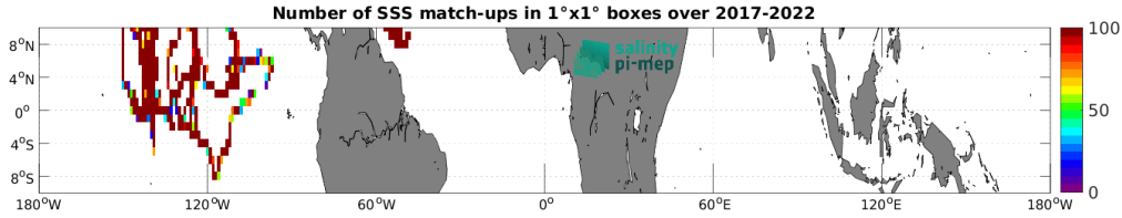
Figure 5: Number of SSS match-ups between Saildrone SSS and the SMOS SSS L3 v335 - 10 Days - 25 km (CATDS-CPDC) SSS product for the Equatorial Ocean 10N-10S Pi-MEP region over 1^\circ \times 1^\circ boxes and for the full satellite product period.
