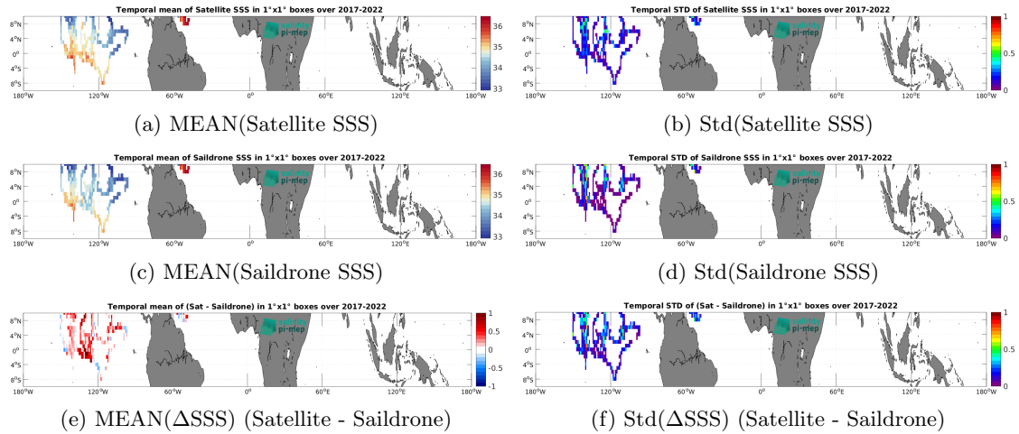
Figure 7: Temporal mean (left) and Std (right) of SSS from SMOS SSS L3 v335 - 10 Days - 25 km (CATDS-CPDC) (top), Saildrone (middle), and of \Delta SSS (Satellite - Saildrone). Only match-up pairs are used to generate these maps.
