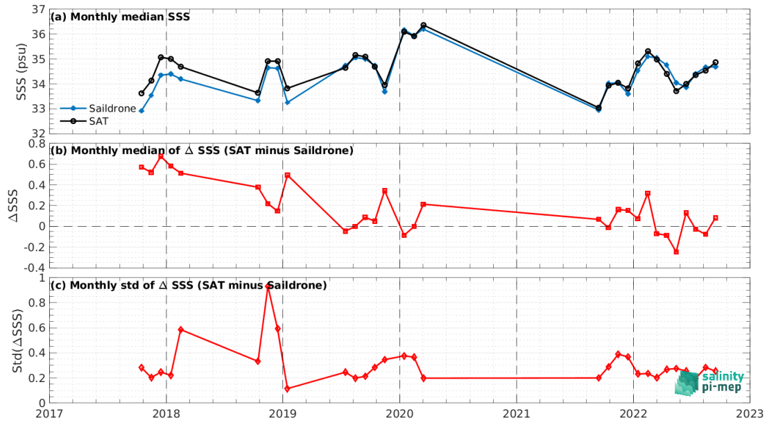
Figure 7: Time series of the monthly median SSS (top), median of \Delta SSS (Satellite - Sairdron) and Std of \Delta SSS (Satellite - Sairdron) over the Equatorial Ocean 10N-10S Pi-MEP region considering all match-ups collected by the Pi-MEP.
