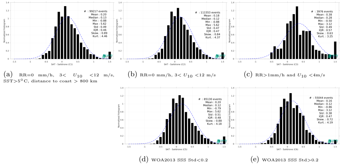
Figure 13: Normalized histogram of \Delta SSS (SMOS SSS L3 v335 - 10 Days - 25 km (CATDS-CPDC) - Saildrone) for 5 different subdatasets corresponding to: RR=0 mm/h, 3 < U_{10} < 12 m/s, SST >5^\circ C, distance to coast > 800 km (a), RR=0 mm/h, 3 < U_{10} < 12 m/s (b), RR >1 mm/h and U_{10} < 4 m/s (c), WOA2013 SSS Std <0.2 (d), WOA2013 SSS Std >0.2 (e).
