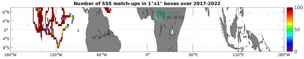
Figure 4: Number of SSS match-ups between Saildrone SSS and the SMOS SSS L3 v335 - 10 Days - 25 km (CATDS-CPDC) SSS product for the Equatorial Ocean 10N-10S Pi-MEP region over 1^\circ \times 1^\circ boxes and for the full satellite product period.
