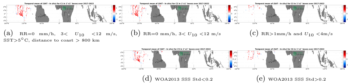
Figure 12: Temporal mean gridded over spatial boxes of size 1^\circ \times 1^\circ of \Delta SSS (SMOS SSS L3 v335 - 10 Days - 25 km (CATDS-CPDC) - Saildrone) for 5 different subdatasets corresponding to: RR=0 mm/h, 3 < U_{10} < 12 m/s, SST>5°C, distance to coast > 800 km (a), RR=0 mm/h, 3 < U_{10} < 12 m/s (b), RR>1mm/h and U_{10} < 4 m/s (c), WOA2013 SSS Std<0.2 (d), WOA2013 SSS Std>0.2 (e).
