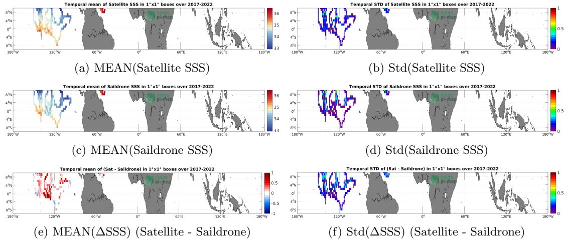
Figure 6: Temporal mean (left) and Std (right) of SSS from SMOS SSS L3 v335 - 10 Days - 25 km (CATDS-CPDC) (top), Saildrone (middle), and of \Delta SSS (Satellite - Saildrone). Only match-up pairs are used to generate these maps.
