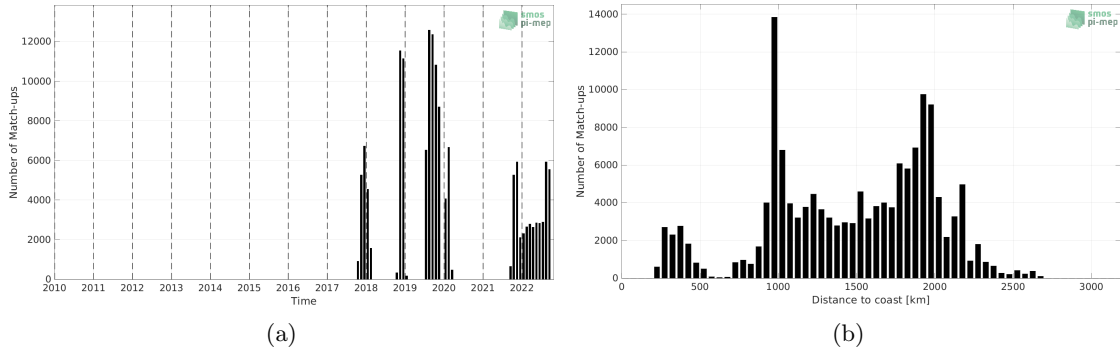
Figure 1: Number of match-ups between Saildrone and SMOS SSS L3 v335 - 10 Days - 25 km (CATDS-CPDC) SSS as a function of time (a) and as function of the distance to coast (b) over the Equatorial Ocean 10N-10S Pi-MEP region and for the full satellite product period.
