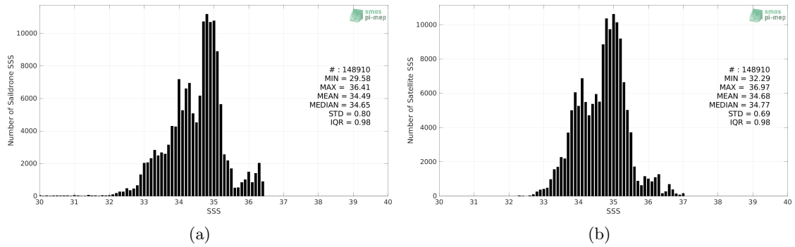
Figure 2: Histograms of SSS from Saildrone (a) and SMOS SSS L3 v335 - 10 Days - 25 km (CATDS-CPDC) (b) considering all match-up pairs per bins of 0.1 over the Equatorial Ocean 10N-10S Pi-MEP region and for the full satellite product period.
