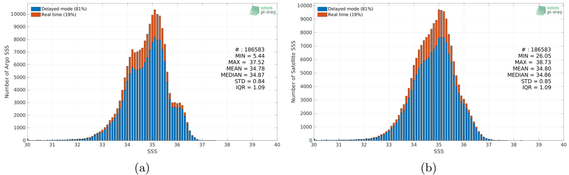
Figure 2: Histograms of SSS from Argo (a) and SMOS SSS L3 v335 - 10 Days - 25 km (CATDS-CPDC) (b) considering all match-up pairs per bins of 0.1 over the Equatorial Ocean 10N-10S Pi-MEP region and for the full satellite product period.
