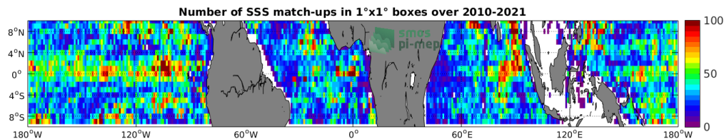
Figure 4: Number of SSS match-ups between Argo SSS and the SMOS SSS L3 v335 - 10 Days - 25 km (CATDS-CPDC) SSS product for the Equatorial Ocean 10N-10S Pi-MEP region over 1^{\circ} \times 1^{\circ} boxes and for the full satellite product period.
