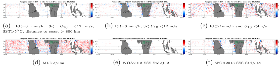
Figure 12: Temporal mean gridded over spatial boxes of size 1^\circ \times 1^\circ of \Delta SSS (SMOS SSS L3 v335 - 10 Days - 25 km (CATDS-CPDC) - Argo) for 6 different subdatasets corresponding to: RR=0 mm/h, 3 < U_{10} < 12 m/s, SST > 5^\circ C , distance to coast > 800 km (a), RR=0 mm/h, 3 < U_{10} < 12 m/s (b), RR > 1 mm/h and U_{10} < 4 m/s (c), MLD < 20 m (d), WOA2013 SSS Std < 0.2 (e), WOA2013 SSS Std > 0.2 (f).
