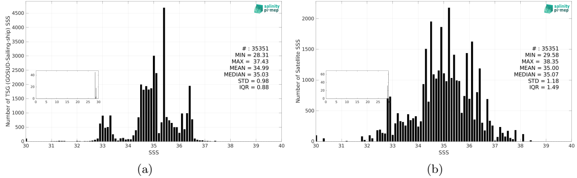
Figure 3: Histograms of SSS from TSG (GOSUD-Sailing-ship) (a) and SMOS SSS L2Q v333 - 0.25 Deg (CATDS-CPDC) (b) considering all match-up pairs per bins of 0.1 over the Equatorial Ocean 10N-10S Pi-MEP region and for the full satellite product period.
