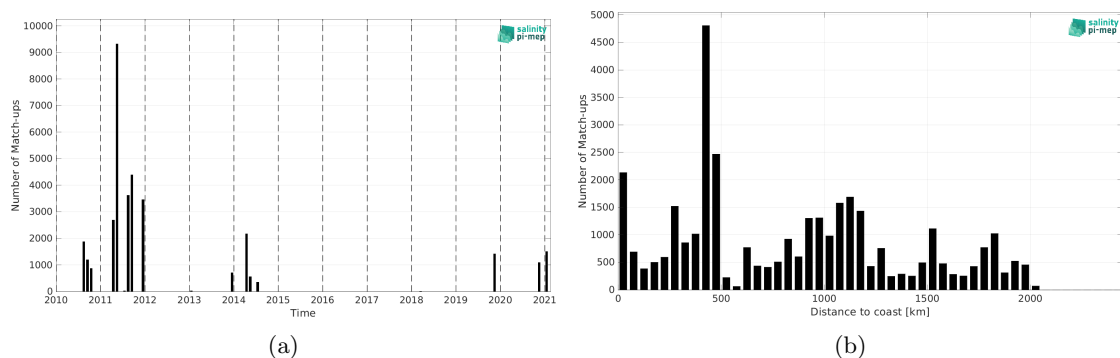
Figure 2: Number of match-ups between TSG (GOSUD-Sailing-ship) and SMOS SSS L2Q v333 - 0.25 Deg (CATDS-CPDC) SSS as a function of time (a) and as function of the distance to coast (b) over the Equatorial Ocean 10N-10S Pi-MEP region and for the full satellite product period.
