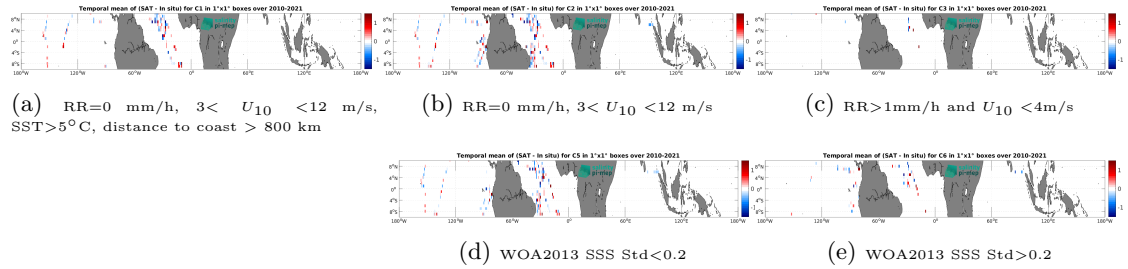
Figure 14: Temporal mean gridded over spatial boxes of size 1^\circ \times 1^\circ of \Delta SSS (SMOS SSS L2Q v333 - 0.25 Deg (CATDS-CPDC) - TSG (GOSUD-Sailing-ship)) for 5 different subdatasets corresponding to:RR=0 mm/h, 3 < U_{10} < 12 m/s, SST>5°C, distance to coast > 800 km (a), RR=0 mm/h, 3 < U_{10} < 12 m/s (b), RR>1mm/h and U_{10} < 4 m/s (c), WOA2013 SSS Std<0.2 (d), WOA2013 SSS Std>0.2 (e).
