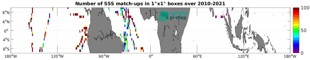
Figure 5: Number of SSS match-ups between TSG (GOSUD-Sailing-ship) SSS and the SMOS SSS L2Q v333 - 0.25 Deg (CATDS-CPDC) SSS product for the Equatorial Ocean 10N-10S Pi-MEP region over 1^\circ \times 1^\circ boxes and for the full satellite product period.
