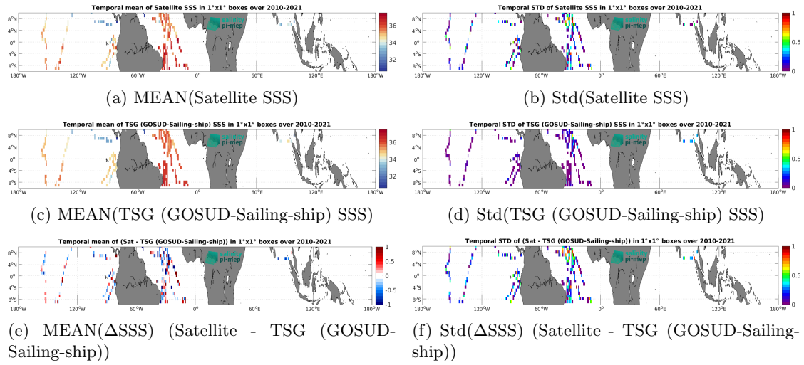
Figure 7: Temporal mean (left) and Std (right) of SSS from SMOS SSS L2Q v333 - 0.25 Deg (CATDS-CPDC) (top), TSG (GOSUD-Sailing-ship) (middle), and of \Delta SSS (Satellite - TSG (GOSUD-Sailing-ship)). Only match-up pairs are used to generate these maps.
