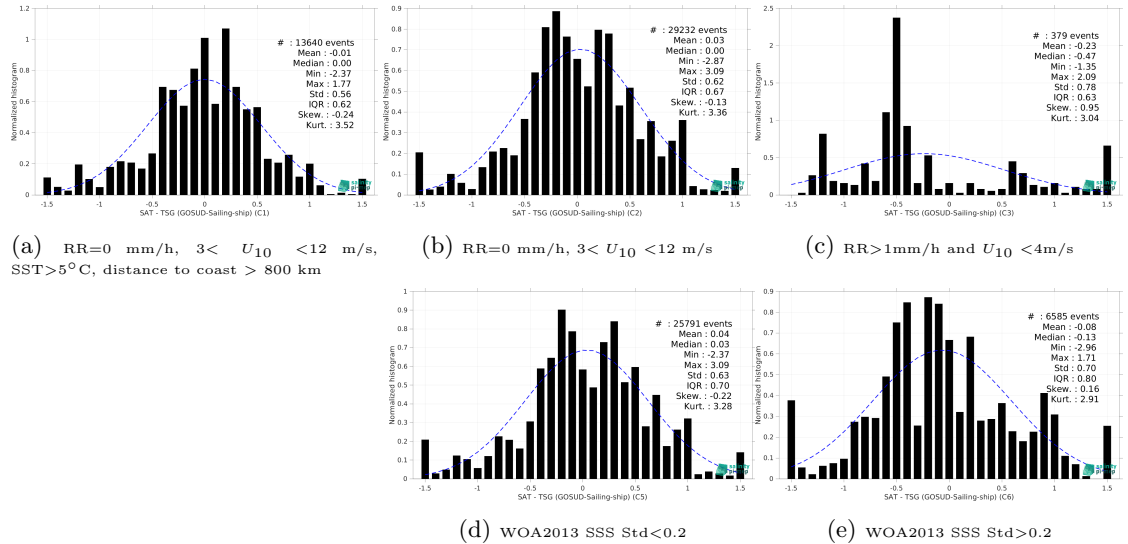
Figure 15: Normalized histogram of \Delta\text{SSS} (SMOS SSS L2Q v333 - 0.25 Deg (CATDS-CPDC) - TSG (GOSUD-Sailing-ship)) for 5 different subdatasets corresponding to: RR=0 mm/h, 3 < U_{10} < 12 m/s, SST>5°C, distance to coast > 800 km (a), RR=0 mm/h, 3 < U_{10} < 12 m/s (b), RR>1mm/h and U_{10} < 4 m/s (c), WOA2013 SSS Std<0.2 (d), WOA2013 SSS Std>0.2 (e).
