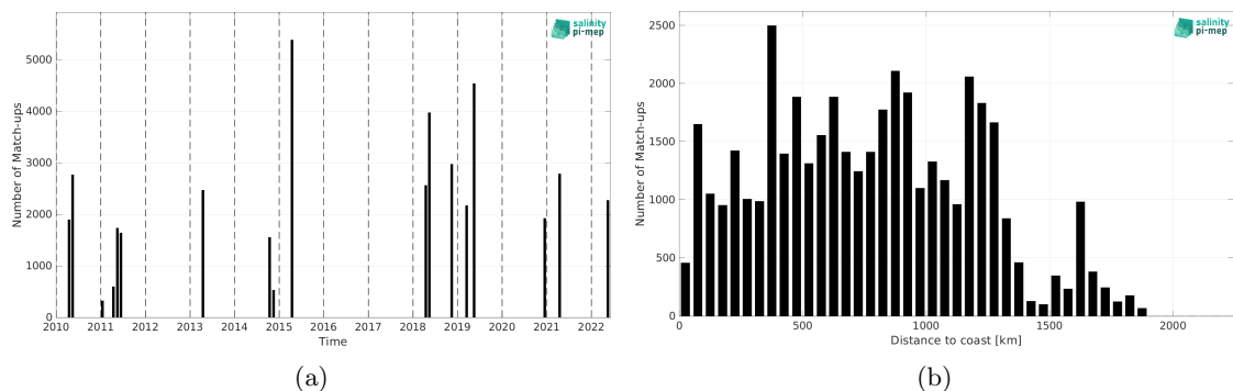
Figure 2: Number of match-ups between TSG (CSIC-UTM) and SMOS SSS L2Q v333 - 0.25 Deg (CATDS-CPDC) SSS as a function of time (a) and as function of the distance to coast (b) over the Equatorial Ocean 10N-10S Pi-MEP region and for the full satellite product period.
