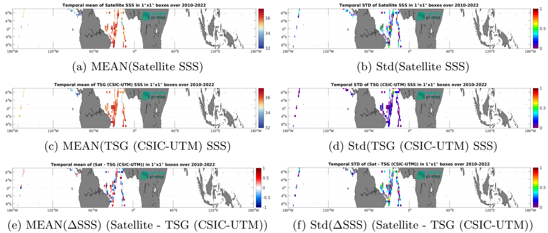
Figure 7: Temporal mean (left) and Std (right) of SSS from SMOS SSS L2Q v333 - 0.25 Deg (CATDS-CPDC) (top), TSG (CSIC-UTM) (middle), and of \Delta SSS (Satellite - TSG (CSIC-UTM)). Only match-up pairs are used to generate these maps.
