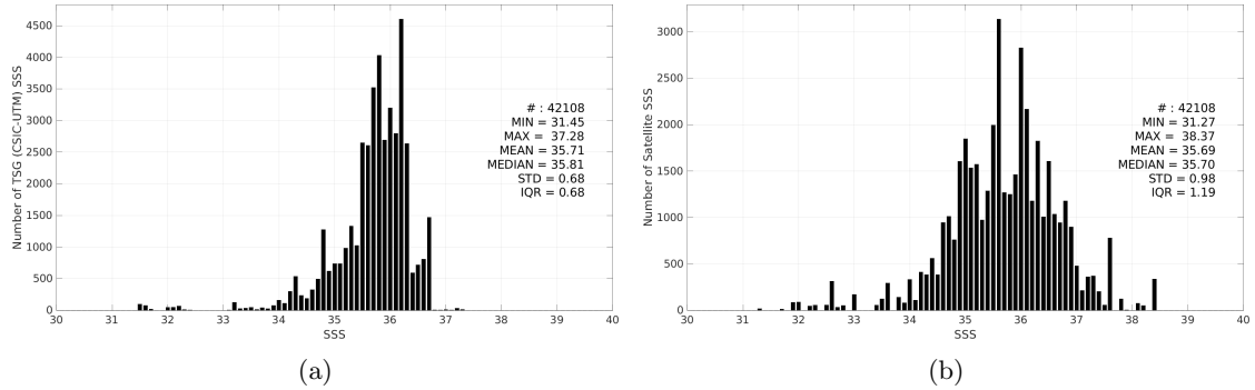
Figure 3: Histograms of SSS from TSG (CSIC-UTM) (a) and SMOS SSS L2Q v333 - 0.25 Deg (CATDS-CPDC) (b) considering all match-up pairs per bins of 0.1 over the Equatorial Ocean 10N-10S Pi-MEP region and for the full satellite product period.
