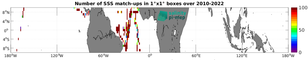
Figure 5: Number of SSS match-ups between TSG (CSIC-UTM) SSS and the SMOS SSS L2Q v333 - 0.25 Deg (CATDS-CPDC) SSS product for the Equatorial Ocean 10N-10S Pi-MEP region over 1^\circ \times 1^\circ boxes and for the full satellite product period.
