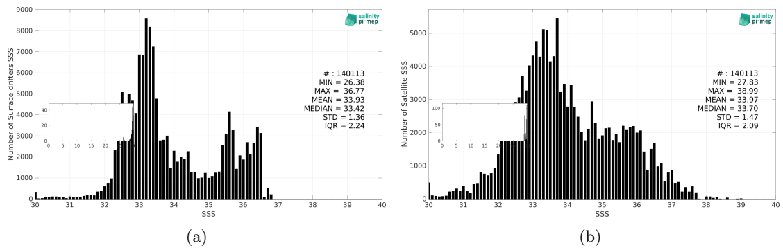
Figure 3: Histograms of SSS from Surface drifters (a) and SMOS SSS L2Q v333 - 0.25 Deg (CATDS-CPDC) (b) considering all match-up pairs per bins of 0.1 over the Equatorial Ocean 10N-10S Pi-MEP region and for the full satellite product period.
