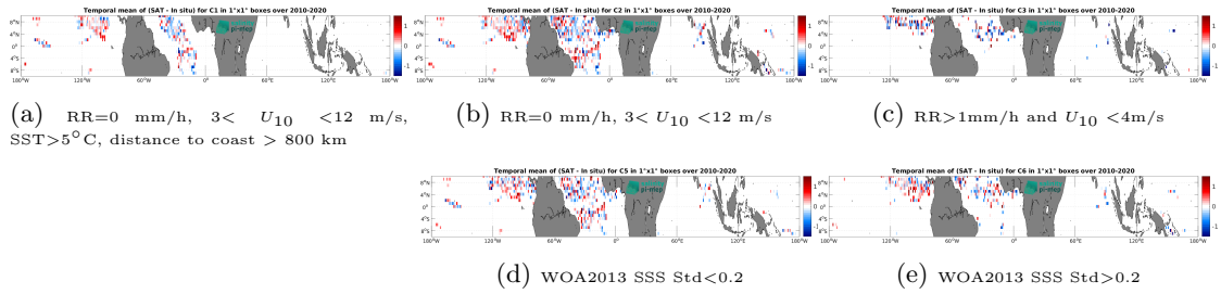
Figure 13: Temporal mean gridded over spatial boxes of size 1^\circ \times 1^\circ of \Delta SSS (SMOS SSS L2Q v333 - 0.25 Deg (CATDS-CPDC) - Surface drifters) for 5 different subdatasets corresponding to: RR=0 mm/h, 3 < U_{10} < 12 m/s, SST >5^\circ C, distance to coast > 800 km (a), RR=0 mm/h, 3 < U_{10} < 12 m/s (b), RR >1 mm/h and U_{10} < 4 m/s (c), WOA2013 SSS Std <0.2 (d), WOA2013 SSS Std >0.2 (e).
