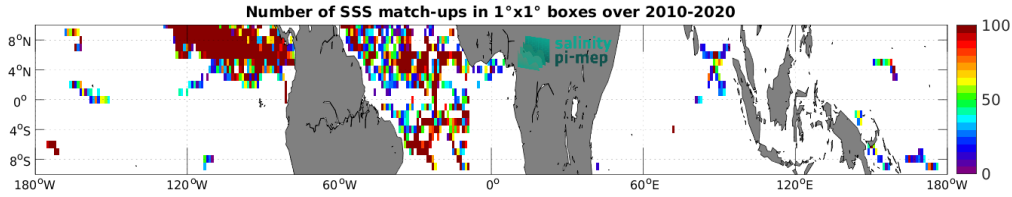
Figure 4: Number of SSS match-ups between Surface drifters SSS and the SMOS SSS L2Q v333 - 0.25 Deg (CATDS-CPDC) SSS product for the Equatorial Ocean 10N-10S Pi-MEP region over 1^\circ \times 1^\circ boxes and for the full satellite product period.
