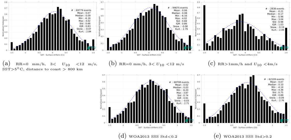
Figure 14: Normalized histogram of \Delta SSS (SMOS SSS L2Q v333 - 0.25 Deg (CATDS-CPDC) - Surface drifters) for 5 different subdatasets corresponding to: RR=0 mm/h, 3 < U_{10} < 12 m/s, SST >5^\circ C, distance to coast > 800 km (a), RR=0 mm/h, 3 < U_{10} < 12 m/s (b), RR >1 mm/h and U_{10} < 4 m/s (c), WOA2013 SSS Std <0.2 (d), WOA2013 SSS Std >0.2 (e).
