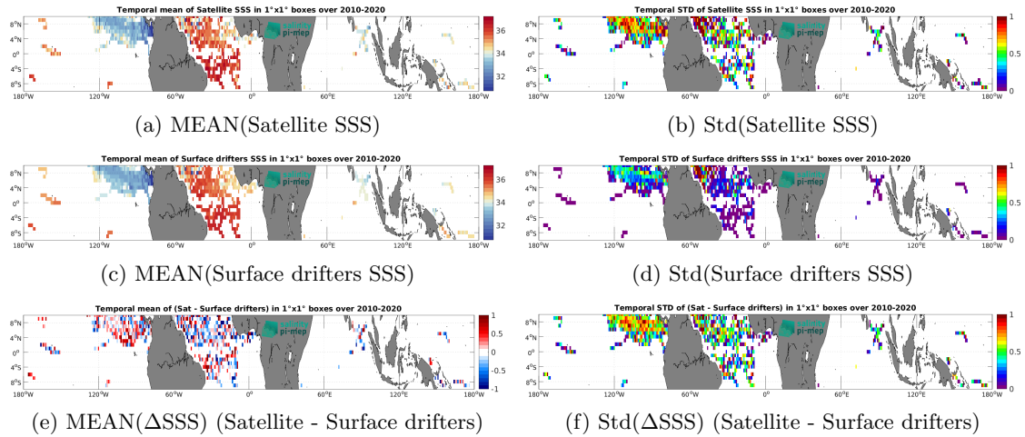
Figure 6: Temporal mean (left) and Std (right) of SSS from SMOS SSS L2Q v333 - 0.25 Deg (CATDS-CPDC) (top), Surface drifters (middle), and of \Delta SSS (Satellite - Surface drifters). Only match-up pairs are used to generate these maps.
