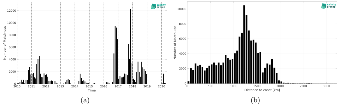
Figure 2: Number of match-ups between Surface drifters and SMOS SSS L2Q v333 - 0.25 Deg (CATDS-CPDC) SSS as a function of time (a) and as function of the distance to coast (b) over the Equatorial Ocean 10N-10S Pi-MEP region and for the full satellite product period.
