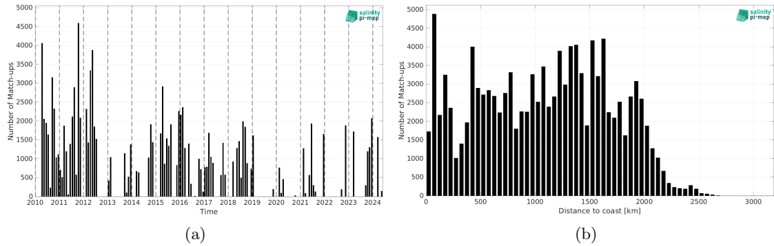
Figure 2: Number of match-ups between TSG (SAMOS) and SMOS SSS L3 v332 - 9 Days (CATDS-CPDC) SSS as a function of time (a) and as function of the distance to coast (b) over the Equatorial Ocean 10N-10S Pi-MEP region and for the full satellite product period.
