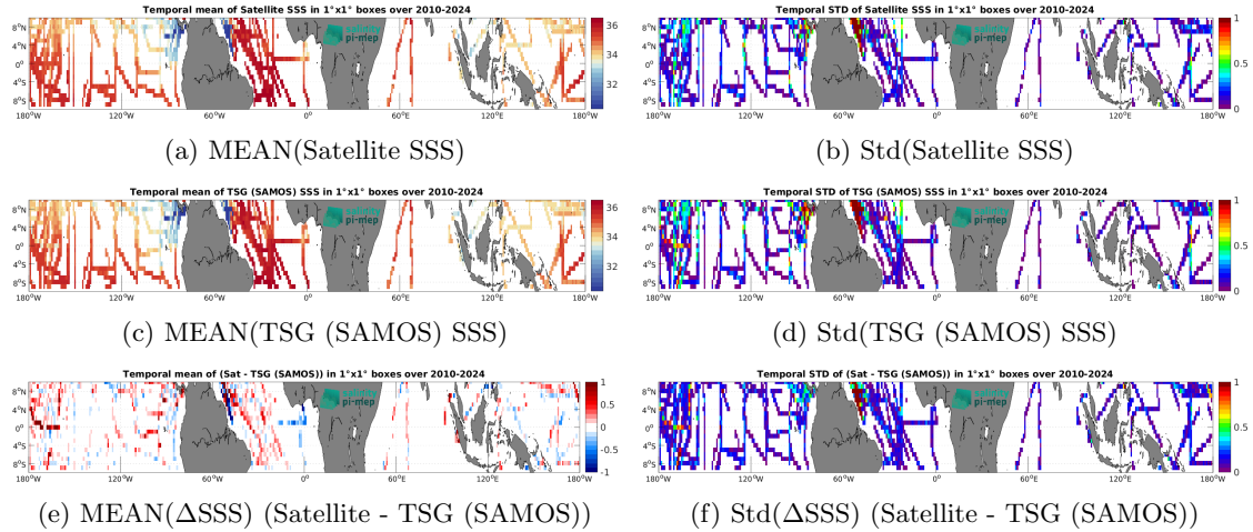
Figure 7: Temporal mean (left) and Std (right) of SSS from SMOS SSS L3 v332 - 9 Days (CATDS-CPDC) (top), TSG (SAMOS) (middle), and of \Delta SSS (Satellite - TSG (SAMOS)). Only match-up pairs are used to generate these maps.
