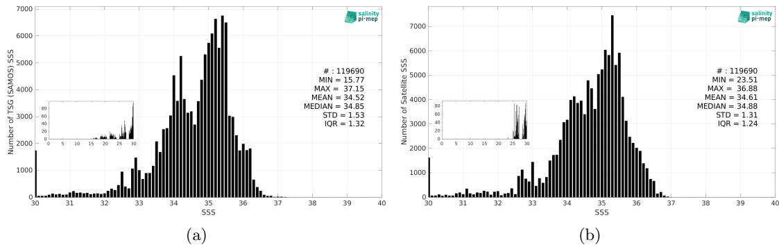
Figure 3: Histograms of SSS from TSG (SAMOS) (a) and SMOS SSS L3 v332 - 9 Days (CATDS-CPDC) (b) considering all match-up pairs per bins of 0.1 over the Equatorial Ocean 10N-10S Pi-MEP region and for the full satellite product period.
