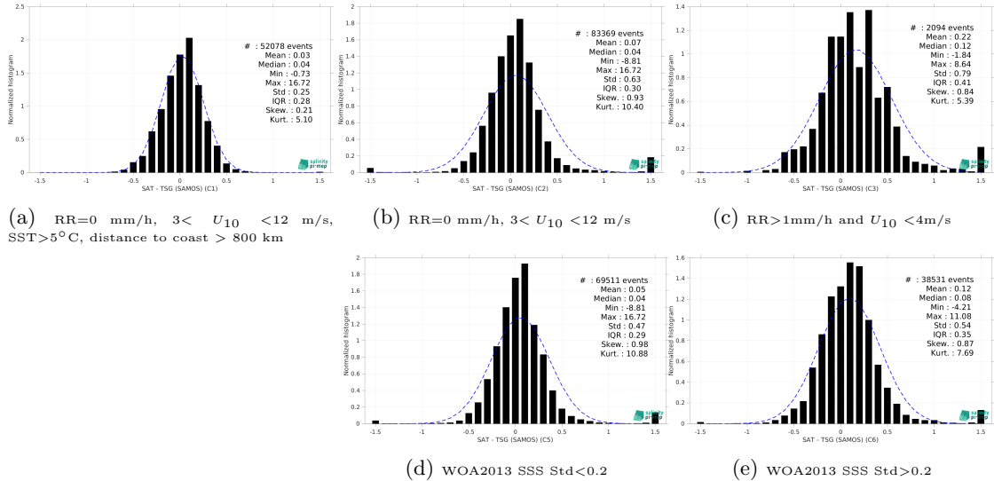
Figure 15: Normalized histogram of \Delta\text{SSS} (SMOS SSS L3 v332 - 9 Days (CATDS-CPDC) - TSG (SAMOS)) for 5 different subdatasets corresponding to: RR=0 mm/h, 3 < U_{10} < 12 m/s, SST>5°C, distance to coast > 800 km (a), RR=0 mm/h, 3 < U_{10} < 12 m/s (b), RR>1mm/h and U_{10} < 4 m/s (c), WOA2013 SSS Std<0.2 (d), WOA2013 SSS Std>0.2 (e).
