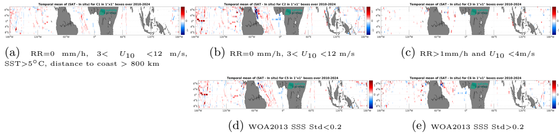
Figure 14: Temporal mean gridded over spatial boxes of size 1^\circ \times 1^\circ of \Delta\text{SSS} (SMOS SSS L3 v332 - 9 Days (CATDS-CPDC) - TSG (SAMOS)) for 5 different subdatasets corresponding to: RR=0 mm/h, 3 < U_{10} < 12 m/s, SST>5°C, distance to coast > 800 km (a), RR=0 mm/h, 3 < U_{10} < 12 m/s (b), RR>1mm/h and U_{10} < 4 m/s (c), WOA2013 SSS Std<0.2 (d), WOA2013 SSS Std>0.2 (e).
