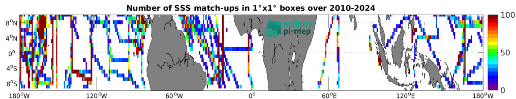
Figure 5: Number of SSS match-ups between TSG (SAMOS) SSS and the SMOS SSS L3 v332 - 9 Days (CATDS-CPDC) SSS product for the Equatorial Ocean 10N-10S Pi-MEP region over 1^\circ \times 1^\circ boxes and for the full satellite product period.
