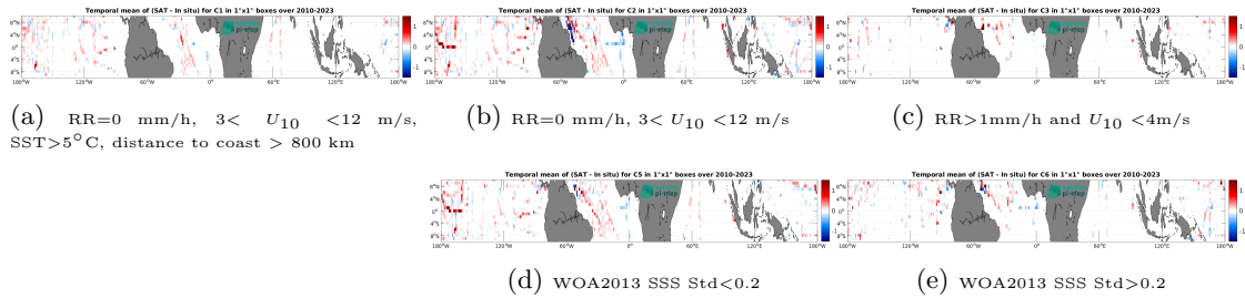
Figure 12: Temporal mean gridded over spatial boxes of size 1^\circ \times 1^\circ of \Delta SSS (SMOS SSS L3 v332 - 9 Days (CATDS-CPDC) - TSG (SAMOS)) for 5 different subdatasets corresponding to:RR=0 mm/h, 3 < U_{10} < 12 m/s, SST >5^\circ\text{C} , distance to coast > 800 km (a), RR=0 mm/h, 3 < U_{10} < 12 m/s (b), RR >1 mm/h and U_{10} < 4 m/s (c), WOA2013 SSS Std <0.2 (d), WOA2013 SSS Std >0.2 (e).
