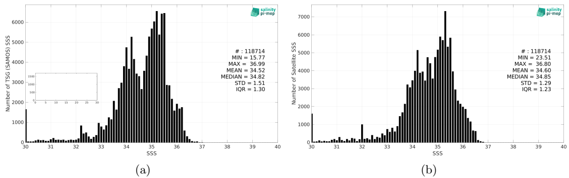
Figure 2: Histograms of SSS from TSG (SAMOS) (a) and SMOS SSS L3 v332 - 9 Days (CATDS-CPDC) (b) considering all match-up pairs per bins of 0.1 over the Equatorial Ocean 10N-10S Pi-MEP region and for the full satellite product period.
