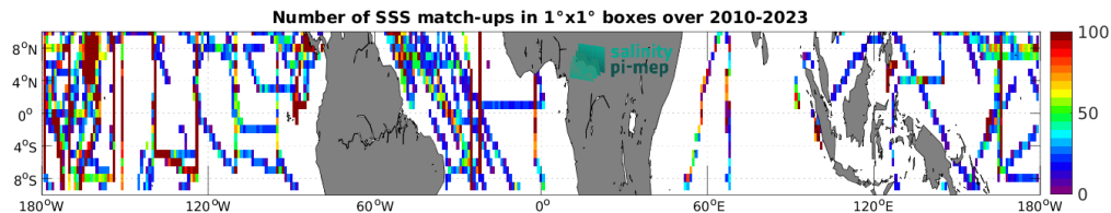
Figure 4: Number of SSS match-ups between TSG (SAMOS) SSS and the SMOS SSS L3 v332 - 9 Days (CATDS-CPDC) SSS product for the Equatorial Ocean 10N-10S Pi-MEP region over 1^\circ \times 1^\circ boxes and for the full satellite product period.
