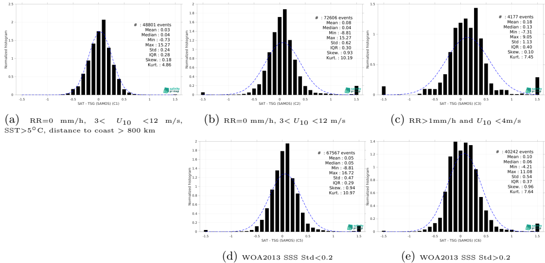
Figure 13: Normalized histogram of \Delta SSS (SMOS SSS L3 v332 - 9 Days (CATDS-CPDC) - TSG (SAMOS)) for 5 different subdatasets corresponding to: RR=0 mm/h, 3 < U_{10} < 12 m/s, SST >5^\circ\text{C} , distance to coast > 800 km (a), RR=0 mm/h, 3 < U_{10} < 12 m/s (b), RR >1 mm/h and U_{10} < 4 m/s (c), WOA2013 SSS Std <0.2 (d), WOA2013 SSS Std >0.2 (e).
