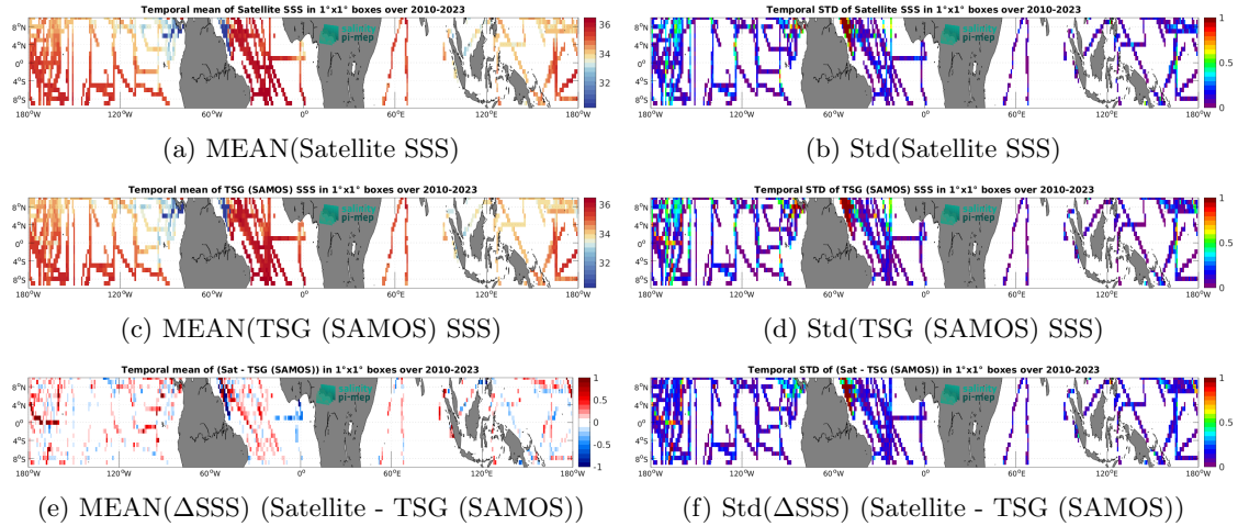
Figure 6: Temporal mean (left) and Std (right) of SSS from SMOS SSS L3 v332 - 9 Days (CATDS-CPDC) (top), TSG (SAMOS) (middle), and of \Delta SSS (Satellite - TSG (SAMOS)). Only match-up pairs are used to generate these maps.
