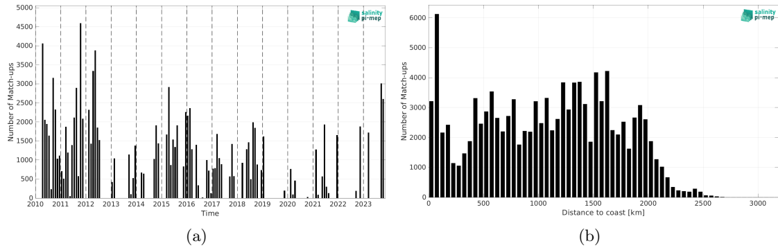
Figure 1: Number of match-ups between TSG (SAMOS) and SMOS SSS L3 v332 - 9 Days (CATDS-CPDC) SSS as a function of time (a) and as function of the distance to coast (b) over the Equatorial Ocean 10N-10S Pi-MEP region and for the full satellite product period.
