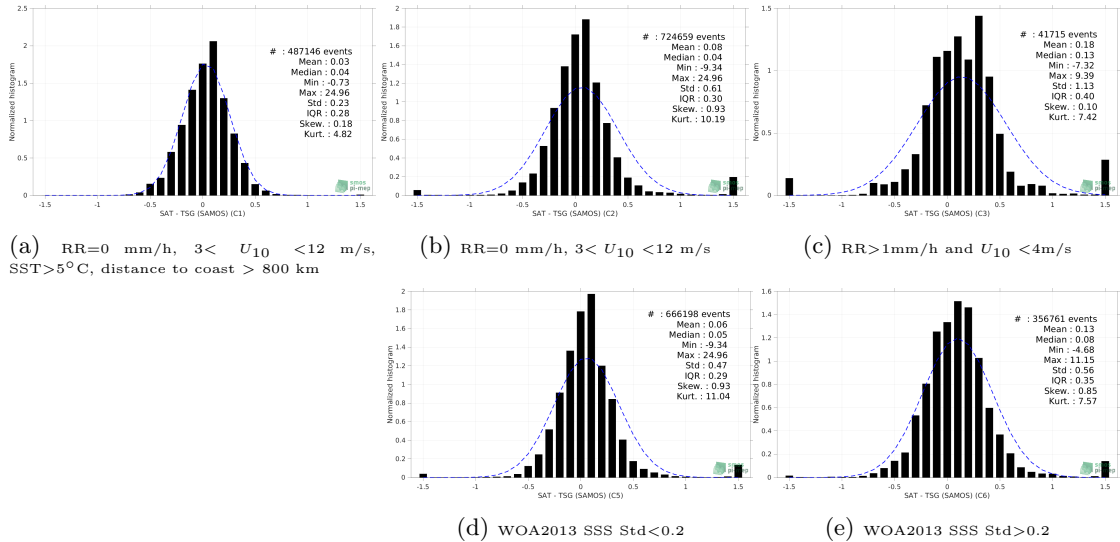
Figure 13: Normalized histogram of \Delta SSS (SMOS SSS L3 v332 - 9 Days (CATDS-CPDC) - TSG (SAMOS)) for 5 different subdatasets corresponding to: RR=0 mm/h, 3 < U_{10} < 12 m/s, SST >5^\circ C, distance to coast > 800 km (a), RR=0 mm/h, 3 < U_{10} < 12 m/s (b), RR >1 mm/h and U_{10} < 4 m/s (c), WOA2013 SSS Std <0.2 (d), WOA2013 SSS Std >0.2 (e).
