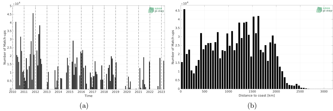
Figure 1: Number of match-ups between TSG (SAMOS) and SMOS SSS L3 v332 - 9 Days (CATDS-CPDC) SSS as a function of time (a) and as function of the distance to coast (b) over the Equatorial Ocean 10N-10S Pi-MEP region and for the full satellite product period.
