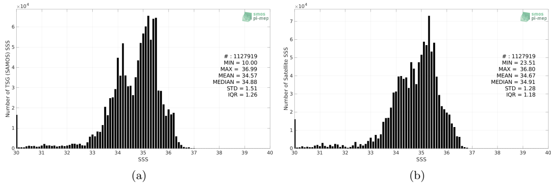
Figure 2: Histograms of SSS from TSG (SAMOS) (a) and SMOS SSS L3 v332 - 9 Days (CATDS-CPDC) (b) considering all match-up pairs per bins of 0.1 over the Equatorial Ocean 10N-10S Pi-MEP region and for the full satellite product period.
