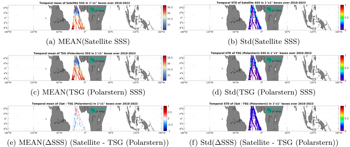
Figure 7: Temporal mean (left) and Std (right) of SSS from SMOS SSS L3 v332 - 9 Days (CATDS-CPDC) (top), TSG (Polarstern) (middle), and of \Delta SSS (Satellite - TSG (Polarstern)). Only match-up pairs are used to generate these maps.
