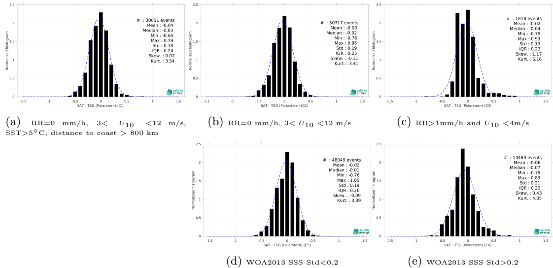
Figure 15: Normalized histogram of \Delta SSS (SMOS SSS L3 v332 - 9 Days (CATDS-CPDC) - TSG (Polarstern)) for 5 different subdatasets corresponding to: RR=0 mm/h, 3 < U_{10} < 12 m/s, SST >5^\circ C, distance to coast > 800 km (a), RR=0 mm/h, 3 < U_{10} < 12 m/s (b), RR >1 mm/h and U_{10} < 4 m/s (c), WOA2013 SSS Std <0.2 (d), WOA2013 SSS Std >0.2 (e).
