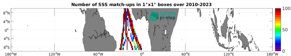
Figure 5: Number of SSS match-ups between TSG (Polarstern) SSS and the SMOS SSS L3 v332 - 9 Days (CATDS-CPDC) SSS product for the Equatorial Ocean 10N-10S Pi-MEP region over 1^\circ \times 1^\circ boxes and for the full satellite product period.
