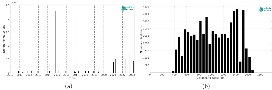
Figure 2: Number of match-ups between TSG (Polarstern) and SMOS SSS L3 v332 - 9 Days (CATDS-CPDC) SSS as a function of time (a) and as function of the distance to coast (b) over the Equatorial Ocean 10N-10S Pi-MEP region and for the full satellite product period.
