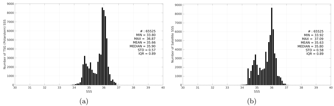
Figure 3: Histograms of SSS from TSG (Polarstern) (a) and SMOS SSS L3 v332 - 9 Days (CATDS-CPDC) (b) considering all match-up pairs per bins of 0.1 over the Equatorial Ocean 10N-10S Pi-MEP region and for the full satellite product period.
