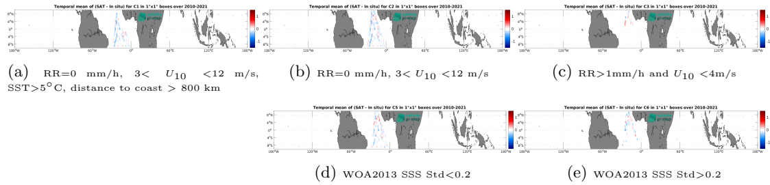
Figure 12: Temporal mean gridded over spatial boxes of size 1^\circ \times 1^\circ of \Delta SSS (SMOS SSS L3 v332 - 9 Days (CATDS-CPDC) - TSG (Polarstern)) for 5 different subdatasets corresponding to: RR=0 mm/h, 3 < U_{10} < 12 m/s, SST >5^\circ C, distance to coast > 800 km (a), RR=0 mm/h, 3 < U_{10} < 12 m/s (b), RR >1 mm/h and U_{10} < 4 m/s (c), WOA2013 SSS Std <0.2 (d), WOA2013 SSS Std >0.2 (e).
