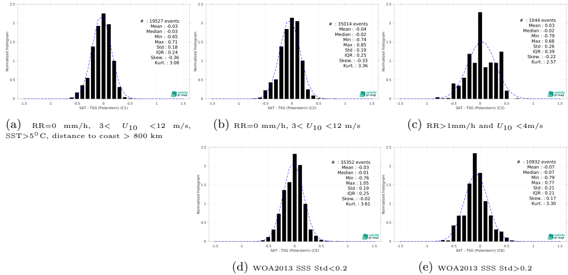
Figure 13: Normalized histogram of \Delta SSS (SMOS SSS L3 v332 - 9 Days (CATDS-CPDC) - TSG (Polarstern)) for 5 different subdatasets corresponding to: RR=0 mm/h, 3 < U_{10} < 12 m/s, SST >5^\circ C, distance to coast > 800 km (a), RR=0 mm/h, 3 < U_{10} < 12 m/s (b), RR >1 mm/h and U_{10} < 4 m/s (c), WOA2013 SSS Std <0.2 (d), WOA2013 SSS Std >0.2 (e).
