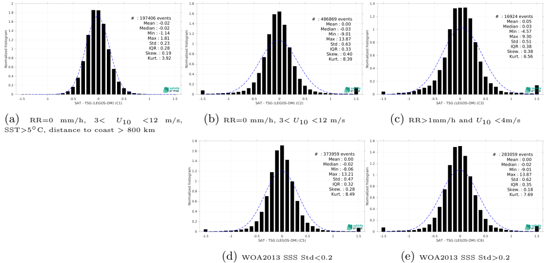
Figure 15: Normalized histogram of \Delta SSS (SMOS SSS L3 v332 - 9 Days (CATDS-CPDC) - TSG (LEGOS-DM)) for 5 different subdatasets corresponding to: RR=0 mm/h, 3 < U_{10} < 12 m/s, SST>5°C, distance to coast > 800 km (a), RR=0 mm/h, 3 < U_{10} < 12 m/s (b), RR>1mm/h and U_{10} < 4 m/s (c), WOA2013 SSS Std<0.2 (d), WOA2013 SSS Std>0.2 (e).
