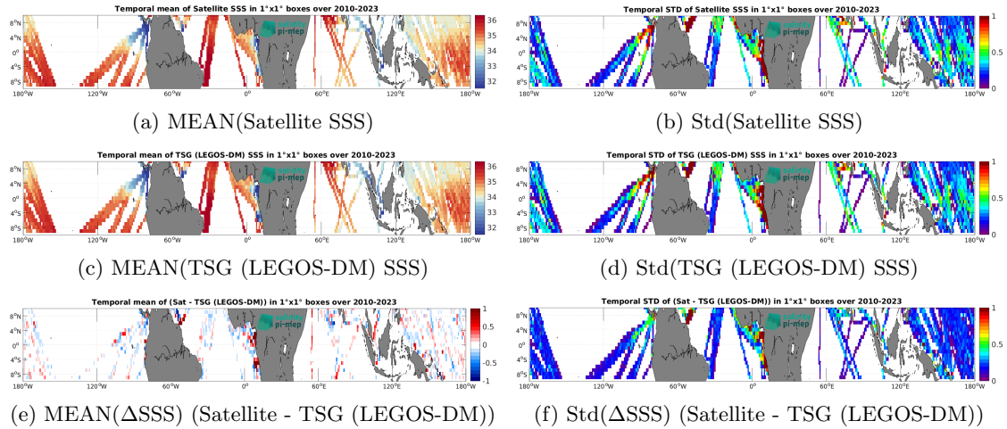
Figure 7: Temporal mean (left) and Std (right) of SSS from SMOS SSS L3 v332 - 9 Days (CATDS-CPDC) (top), TSG (LEGOS-DM) (middle), and of \Delta SSS (Satellite - TSG (LEGOS-DM)). Only match-up pairs are used to generate these maps.
