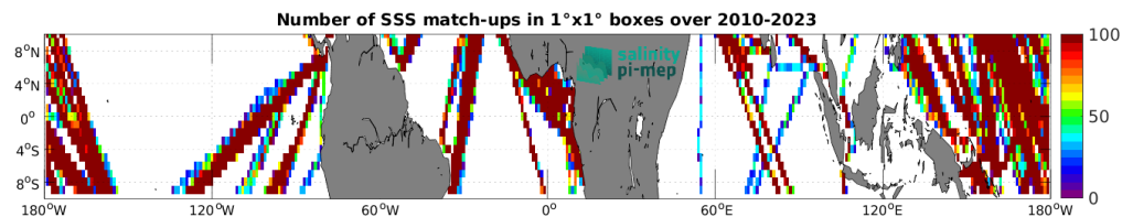
Figure 5: Number of SSS match-ups between TSG (LEGOS-DM) SSS and the SMOS SSS L3 v332 - 9 Days (CATDS-CPDC) SSS product for the Equatorial Ocean 10N-10S Pi-MEP region over 1^\circ \times 1^\circ boxes and for the full satellite product period.
