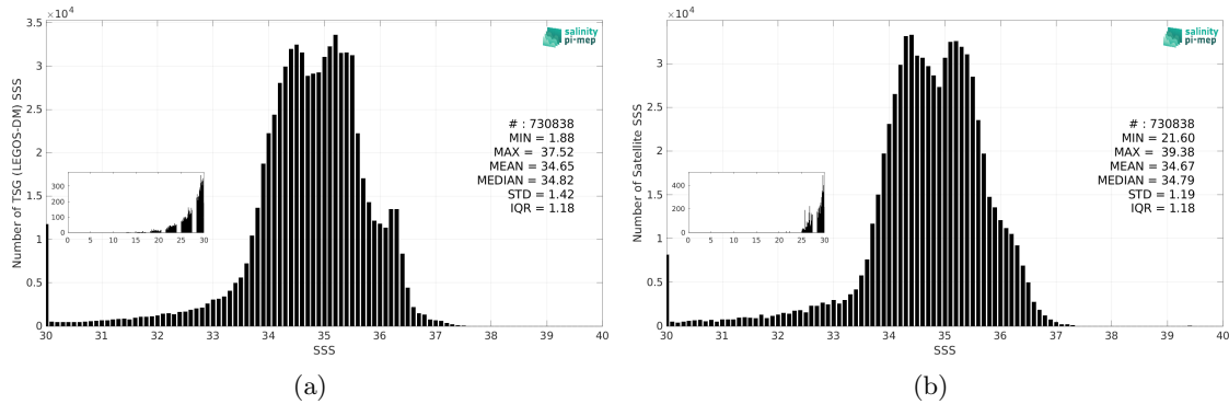
Figure 3: Histograms of SSS from TSG (LEGOS-DM) (a) and SMOS SSS L3 v332 - 9 Days (CATDS-CPDC) (b) considering all match-up pairs per bins of 0.1 over the Equatorial Ocean 10N-10S Pi-MEP region and for the full satellite product period.
