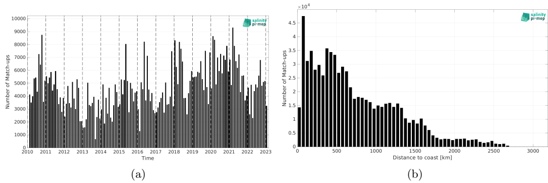
Figure 2: Number of match-ups between TSG (LEGOS-DM) and SMOS SSS L3 v332 - 9 Days (CATDS-CPDC) SSS as a function of time (a) and as function of the distance to coast (b) over the Equatorial Ocean 10N-10S Pi-MEP region and for the full satellite product period.
