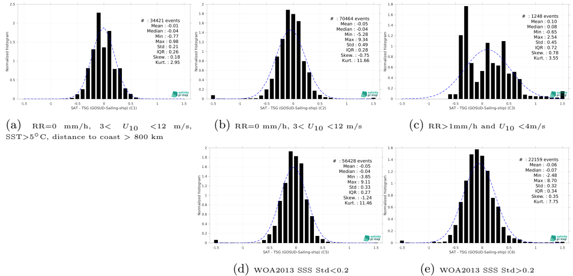
Figure 15: Normalized histogram of \Delta SSS (SMOS SSS L3 v332 - 9 Days (CATDS-CPDC) - TSG (GOSUD-Sailing-ship)) for 5 different subdatasets corresponding to: RR=0 mm/h, 3 < U_{10} < 12 m/s, SST>5°C, distance to coast > 800 km (a), RR=0 mm/h, 3 < U_{10} < 12 m/s (b), RR>1mm/h and U_{10} < 4 m/s (c), WOA2013 SSS Std<0.2 (d), WOA2013 SSS Std>0.2 (e).
