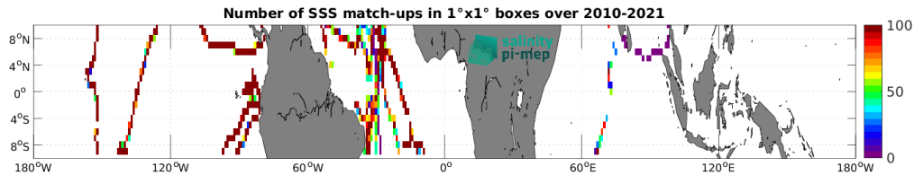
Figure 5: Number of SSS match-ups between TSG (GOSUD-Sailing-ship) SSS and the SMOS SSS L3 v332 - 9 Days (CATDS-CPDC) SSS product for the Equatorial Ocean 10N-10S Pi-MEP region over 1^\circ \times 1^\circ boxes and for the full satellite product period.
