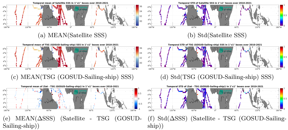
Figure 7: Temporal mean (left) and Std (right) of SSS from SMOS SSS L3 v332 - 9 Days (CATDS-CPDC) (top), TSG (GOSUD-Sailing-ship) (middle), and of \Delta SSS (Satellite - TSG (GOSUD-Sailing-ship)). Only match-up pairs are used to generate these maps.
