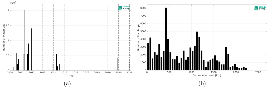
Figure 2: Number of match-ups between TSG (GOSUD-Sailing-ship) and SMOS SSS L3 v332 - 9 Days (CATDS-CPDC) SSS as a function of time (a) and as function of the distance to coast (b) over the Equatorial Ocean 10N-10S Pi-MEP region and for the full satellite product period.
