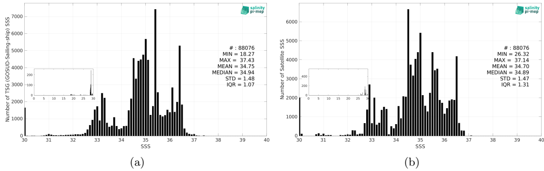
Figure 3: Histograms of SSS from TSG (GOSUD-Sailing-ship) (a) and SMOS SSS L3 v332 - 9 Days (CATDS-CPDC) (b) considering all match-up pairs per bins of 0.1 over the Equatorial Ocean 10N-10S Pi-MEP region and for the full satellite product period.
