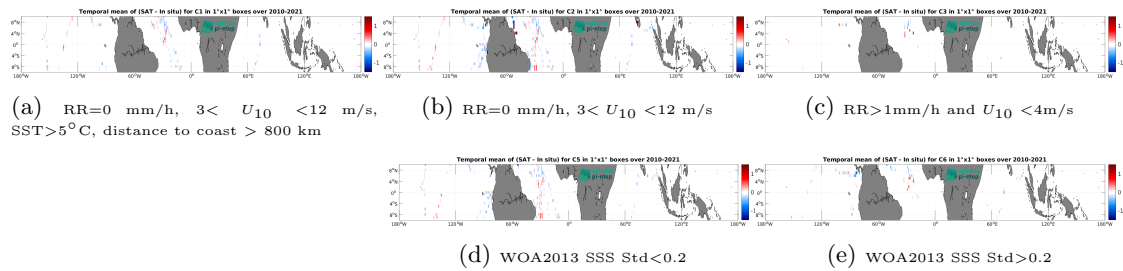
Figure 12: Temporal mean gridded over spatial boxes of size 1^{\circ}\times 1^{\circ} of \Delta SSS (SMOS SSS L3 v332 - 9 Days (CATDS-CPDC) - TSG (GOSUD-Sailing-ship)) for 5 different subdatasets corresponding to:RR=0 mm/h, 3 < U_{10} < 12 m/s, SST >5^{\circ}\text{C} , distance to coast > 800 km (a), RR=0 mm/h, 3 < U_{10} < 12 m/s (b), RR >1 mm/h and U_{10} < 4 m/s (c), WOA2013 SSS Std <0.2 (d), WOA2013 SSS Std >0.2 (e).
