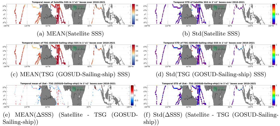
Figure 6: Temporal mean (left) and Std (right) of SSS from SMOS SSS L3 v332 - 9 Days (CATDS-CPDC) (top), TSG (GOSUD-Sailing-ship) (middle), and of \Delta SSS (Satellite - TSG (GOSUD-Sailing-ship)). Only match-up pairs are used to generate these maps.
