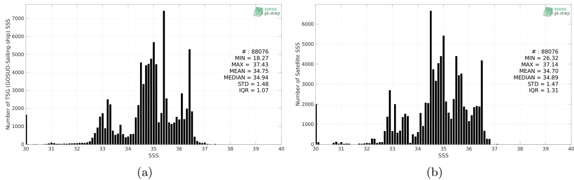
Figure 2: Histograms of SSS from TSG (GOSUD-Sailing-ship) (a) and SMOS SSS L3 v332 - 9 Days (CATDS-CPDC) (b) considering all match-up pairs per bins of 0.1 over the Equatorial Ocean 10N-10S Pi-MEP region and for the full satellite product period.
