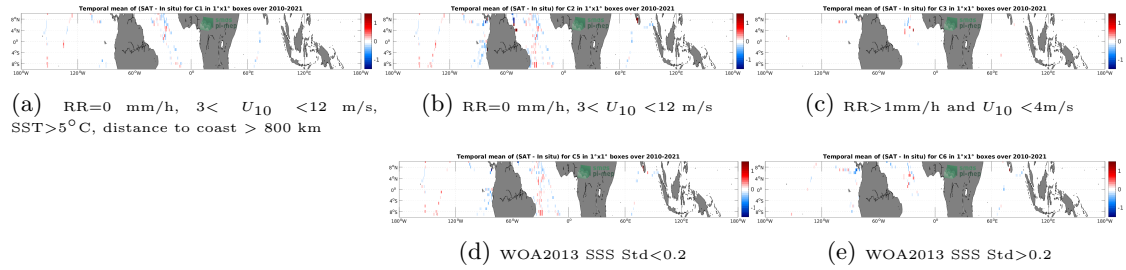
Figure 12: Temporal mean gridded over spatial boxes of size 1^{\circ}\times 1^{\circ} of \Delta SSS (SMOS SSS L3 v332 - 9 Days (CATDS-CPDC) - TSG (GOSUD-Sailing-ship)) for 5 different subdatasets corresponding to:RR=0 mm/h, 3 < U_{10} < 12 m/s, SST >5^{\circ}\text{C} , distance to coast > 800 km (a), RR=0 mm/h, 3 < U_{10} < 12 m/s (b), RR >1 mm/h and U_{10} < 4 m/s (c), WOA2013 SSS Std <0.2 (d), WOA2013 SSS Std >0.2 (e).
