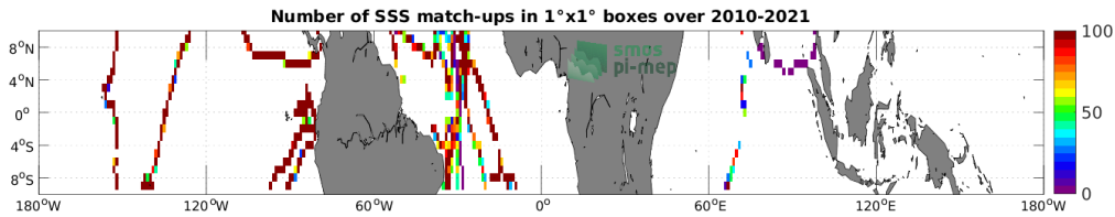
Figure 4: Number of SSS match-ups between TSG (GOSUD-Sailing-ship) SSS and the SMOS SSS L3 v332 - 9 Days (CATDS-CPDC) SSS product for the Equatorial Ocean 10N-10S Pi-MEP region over 1^\circ \times 1^\circ boxes and for the full satellite product period.
