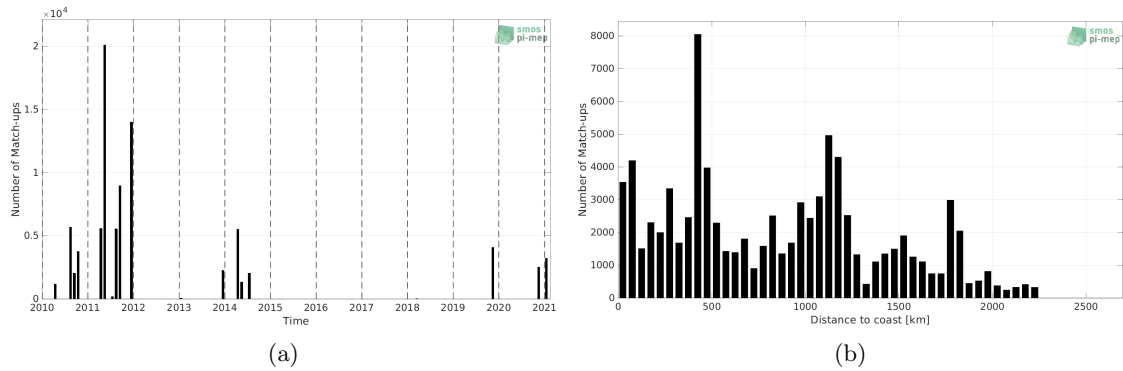
Figure 1: Number of match-ups between TSG (GOSUD-Sailing-ship) and SMOS SSS L3 v332 - 9 Days (CATDS-CPDC) SSS as a function of time (a) and as function of the distance to coast (b) over the Equatorial Ocean 10N-10S Pi-MEP region and for the full satellite product period.
