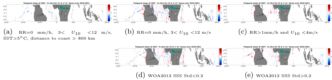
Figure 14: Temporal mean gridded over spatial boxes of size 1^\circ \times 1^\circ of \Delta\text{SSS} (SMOS SSS L3 v332 - 9 Days (CATDS-CPDC) - TSG (GOSUD-Research-vessel)) for 5 different subdatasets corresponding to: RR=0 mm/h, 3 < U_{10} < 12 m/s, SST>5°C, distance to coast > 800 km (a), RR=0 mm/h, 3 < U_{10} < 12 m/s (b), RR>1mm/h and U_{10} < 4 m/s (c), WOA2013 SSS Std<0.2 (d), WOA2013 SSS Std>0.2 (e).
