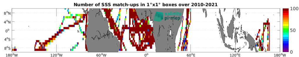
Figure 5: Number of SSS match-ups between TSG (GOSUD-Research-vessel) SSS and the SMOS SSS L3 v332 - 9 Days (CATDS-CPDC) SSS product for the Equatorial Ocean 10N-10S Pi-MEP region over 1^\circ \times 1^\circ boxes and for the full satellite product period.
