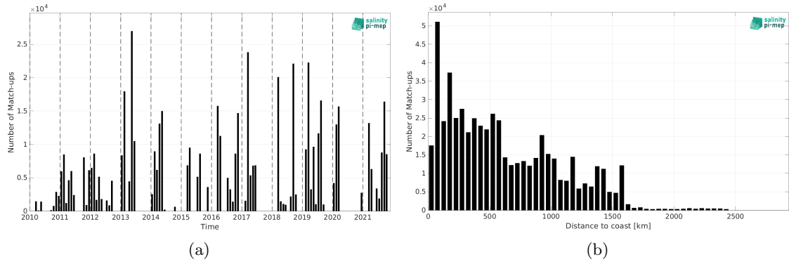
Figure 2: Number of match-ups between TSG (GOSUD-Research-vessel) and SMOS SSS L3 v332 - 9 Days (CATDS-CPDC) SSS as a function of time (a) and as function of the distance to coast (b) over the Equatorial Ocean 10N-10S Pi-MEP region and for the full satellite product period.
