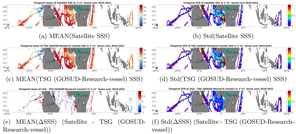
Figure 7: Temporal mean (left) and Std (right) of SSS from SMOS SSS L3 v332 - 9 Days (CATDS-CPDC) (top), TSG (GOSUD-Research-vessel) (middle), and of \Delta SSS (Satellite - TSG (GOSUD-Research-vessel)). Only match-up pairs are used to generate these maps.
