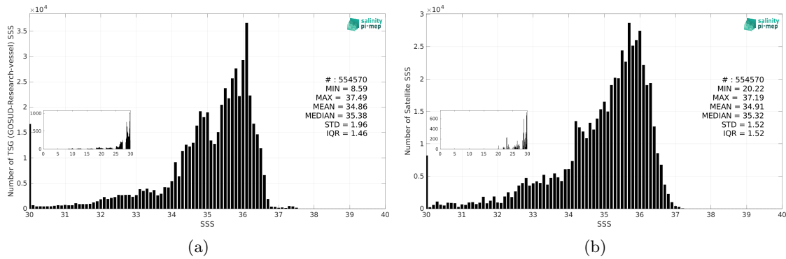
Figure 3: Histograms of SSS from TSG (GOSUD-Research-vessel) (a) and SMOS SSS L3 v332 - 9 Days (CATDS-CPDC) (b) considering all match-up pairs per bins of 0.1 over the Equatorial Ocean 10N-10S Pi-MEP region and for the full satellite product period.
