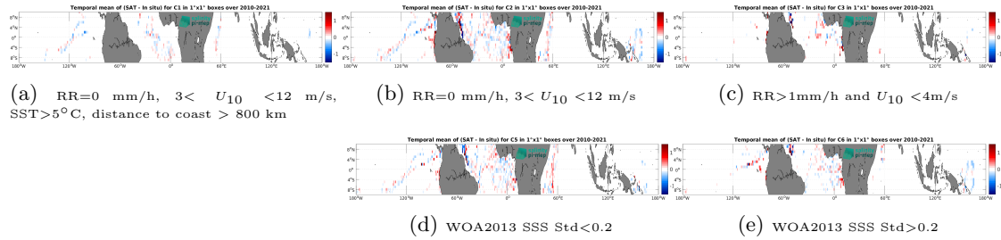
Figure 12: Temporal mean gridded over spatial boxes of size 1^\circ \times 1^\circ of \Delta SSS (SMOS SSS L3 v332 - 9 Days (CATDS-CPDC) - TSG (GOSUD-Research-vessel)) for 5 different subdatasets corresponding to:RR=0 mm/h, 3 < U_{10} < 12 m/s, SST>5°C, distance to coast > 800 km (a), RR=0 mm/h, 3 < U_{10} < 12 m/s (b), RR>1mm/h and U_{10} < 4 m/s (c), WOA2013 SSS Std<0.2 (d), WOA2013 SSS Std>0.2 (e).
