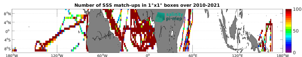
Figure 4: Number of SSS match-ups between TSG (GOSUD-Research-vessel) SSS and the SMOS SSS L3 v332 - 9 Days (CATDS-CPDC) SSS product for the Equatorial Ocean 10N-10S Pi-MEP region over 1^\circ \times 1^\circ boxes and for the full satellite product period.
