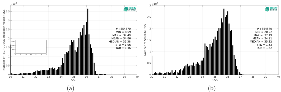
Figure 2: Histograms of SSS from TSG (GOSUD-Research-vessel) (a) and SMOS SSS L3 v332 - 9 Days (CATDS-CPDC) (b) considering all match-up pairs per bins of 0.1 over the Equatorial Ocean 10N-10S Pi-MEP region and for the full satellite product period.
