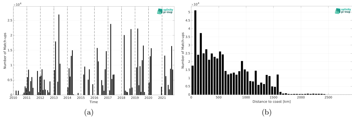
Figure 1: Number of match-ups between TSG (GOSUD-Research-vessel) and SMOS SSS L3 v332 - 9 Days (CATDS-CPDC) SSS as a function of time (a) and as function of the distance to coast (b) over the Equatorial Ocean 10N-10S Pi-MEP region and for the full satellite product period.
